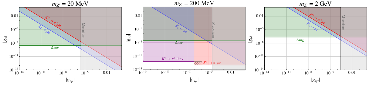
Fig. 25: Constraints on Z' flavor-violating couplings to quarks, g_{sd} , and leptons, g_{e\mu} . Red and blue lines represent the bounds from current limits on \mathcal{B}(K^+ \rightarrow \pi^+ \mu^+ e^+) and \mathcal{B}(K_L \rightarrow \mu^\pm e^\mp) , respectively (Section 4.17). Green and black lines show the bounds from K - \bar{K} and M - \bar{M} mixing, respectively. The hatched region in the central plot shows the range of g_{e\mu} values that could include displaced Z' vertex decays.
