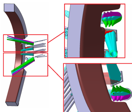
Figure 19. Path of the ECH electromagnetic waves.
