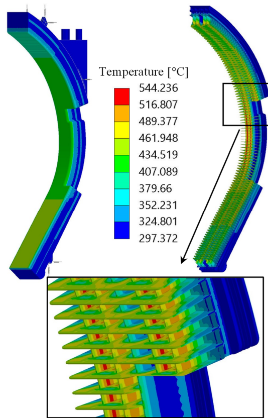
Figure 23. The imposed 3D thermal field.
