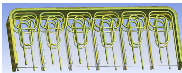
Figure 8. Helical-shaped DWT layout in the COB segment.
