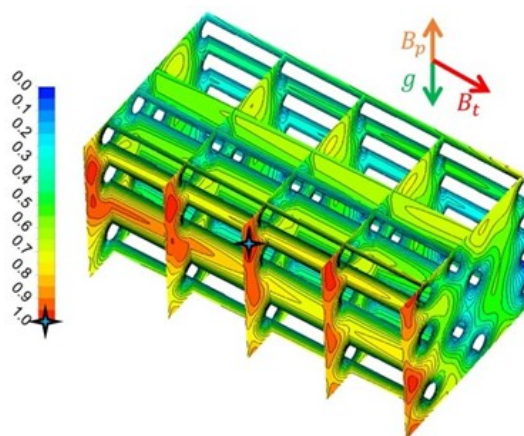
Figure 14. Scaled temperature distribution ( (T-T_{min})/(T_{max}-T_{min}) ) in different planes.
