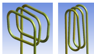
Figure 9. DWT-1 (left) and DWT-2 (right) layout.
