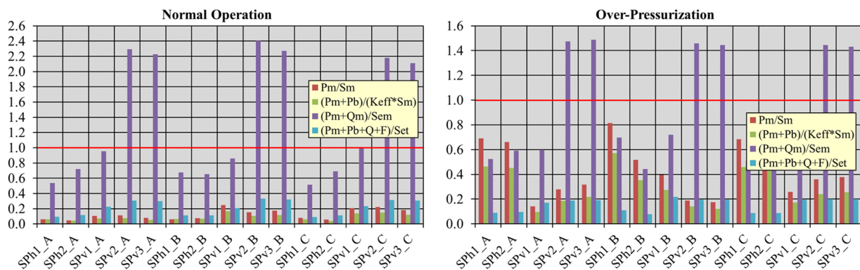
Figure 26. RCC-MRx criteria verification under NO (left) and OP scenarios (right).
