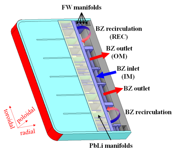
Figure 2. WCLL BB manifold scheme.
