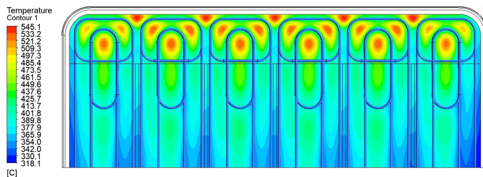
Figure 10. Temperature field on radial-toroidal stiffening plate.
