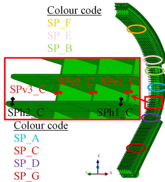
Figure 25. Locations of paths for the stress linearization.
