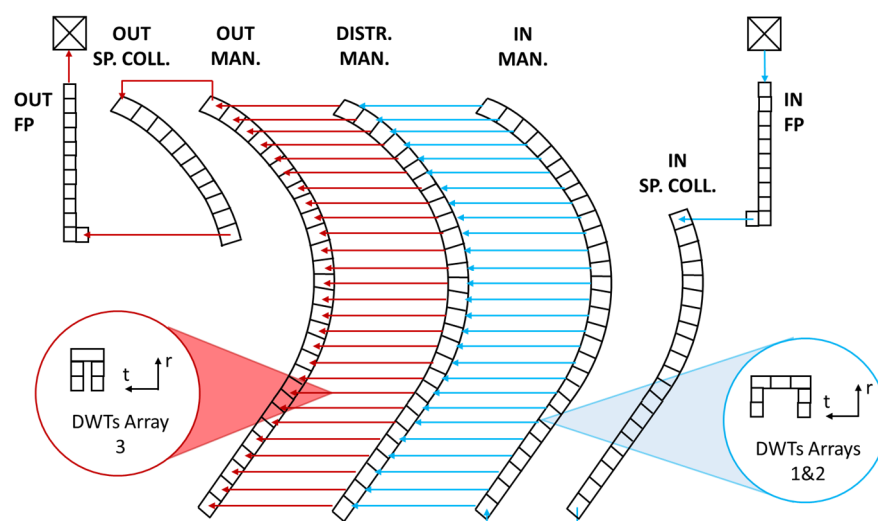
Figure 28. RELAP5/Mod3.3 nodalization of BZ circuit within DEMO WCLL COB segment.
