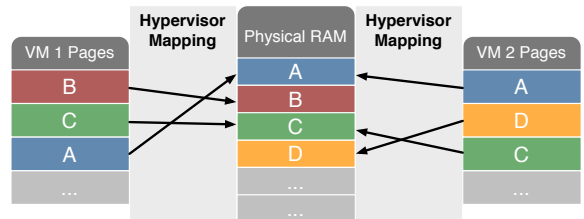
Figure 1: Page sharing between two VMs. The content of a page is indicated by its color/label.
