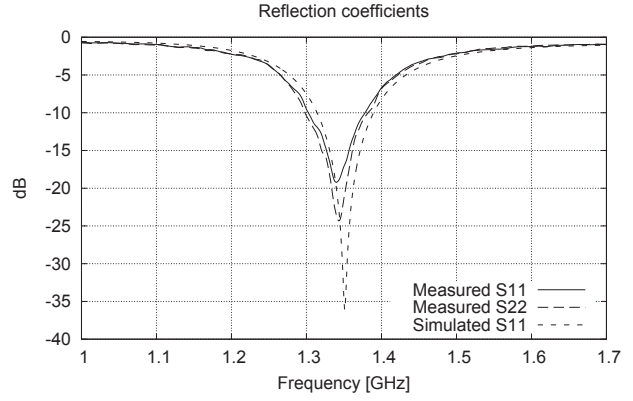
Fig. 3. Measured reflection coefficients
