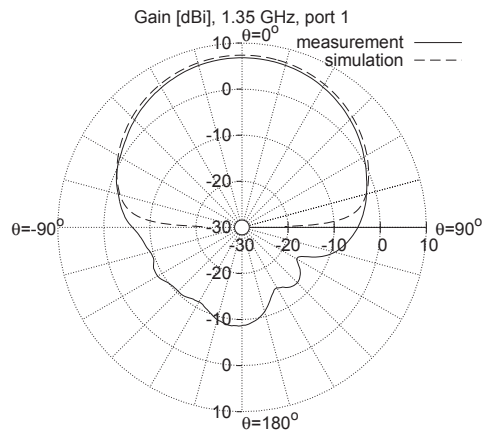
Fig. 4. Simulated and measured gain pattern on the XZ plane, at f = 1.35 GHz, for antenna port 1
