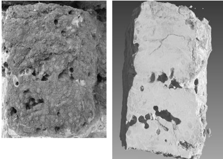
Figure 8. Bioturbated ferruginous sandstone (length: 14 cm ; width: 10 cm) heavily attacked by mason bees (recent perforations marked by light grey clay lining), extracted from the Maagdentoren (left). The corresponding CT-scan (right) shows the original burrows by sea organisms (worm-like faint grey bioturbations), most clearly visible in the upper part of the scan, and similar zones, which attracted the mason bees whose perforations are visible in the middle and the lower part of the scan.
