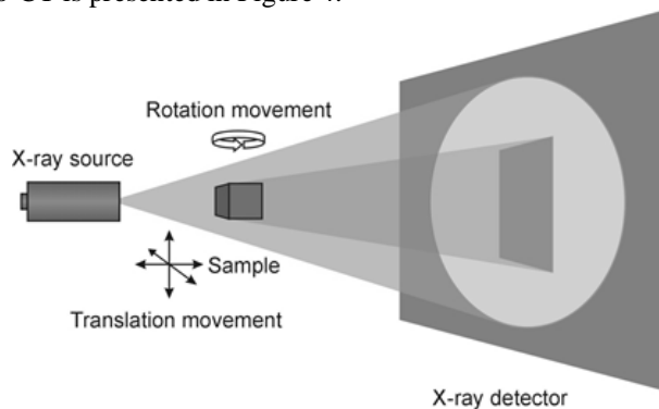
Figure 4. Principle of micro CT.
