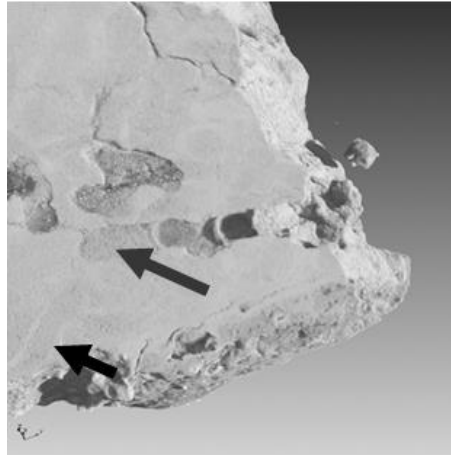
Figure 7. Reconstruction of CT-scans of the outer part of a ferruginous sandstone drillcore. The lower arrow marks a bioturbation dug by burrowing animals during the sedimentation process of the ferruginous sandstone. These bioturbations are characterised by an almost uncemented sand filling, hence of lower density and darker coloured, surrounded by a more strongly cemented rim, hence denser and light coloured. The upper arrow marks a perforation filled with ferruginous sandstone fragments produced during digging of a burrow by a new generation of mason bees. The burrow filled with sandstone fragments is darker coloured indicative for its lower density (size of the image: 4 cm).
