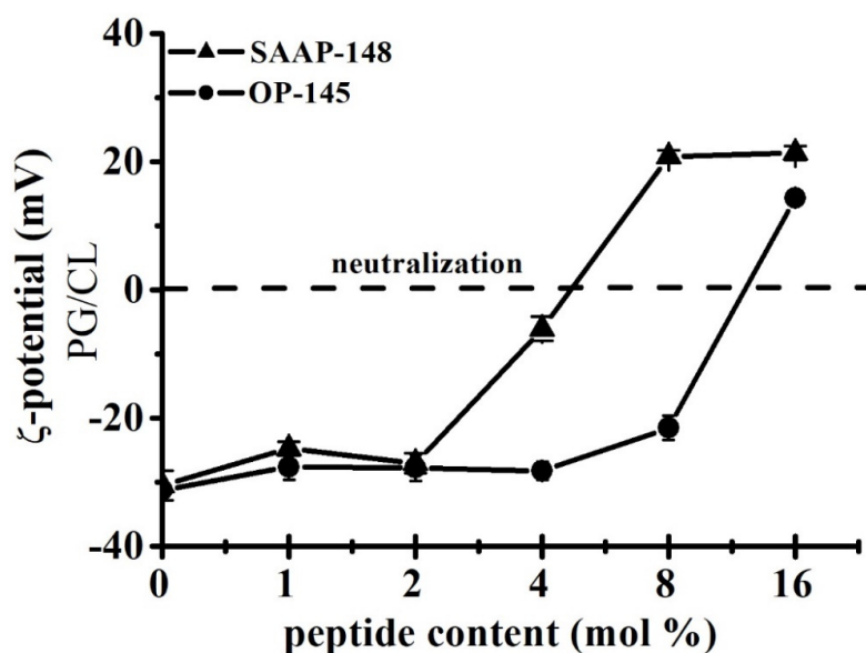
Figure 5. Neutralization of the surface charge of PG/CL membranes by SAAP-148 and OP-145. The \zeta -potential measurements of PG/CL in the presence of SAAP-148 (triangles) and OP-145 (circles) at indicated concentrations ranging from 1 mol% to 16 mol%. Data are summary of three independent experiments. Measurements were performed on the POPG/TOCL mixture as well as on the DMPG/TMCL mixture. There was no difference between POPG/TOCL and DMPG/TMCL measurements in the presence of OP-145. Although a slight difference in concentration dependency is noticed for SAAP-148, the neutralization trend between POPG/TOCL and DMPG/TMCL is similar. Here, only measurements for POPG/TOCL are shown.
