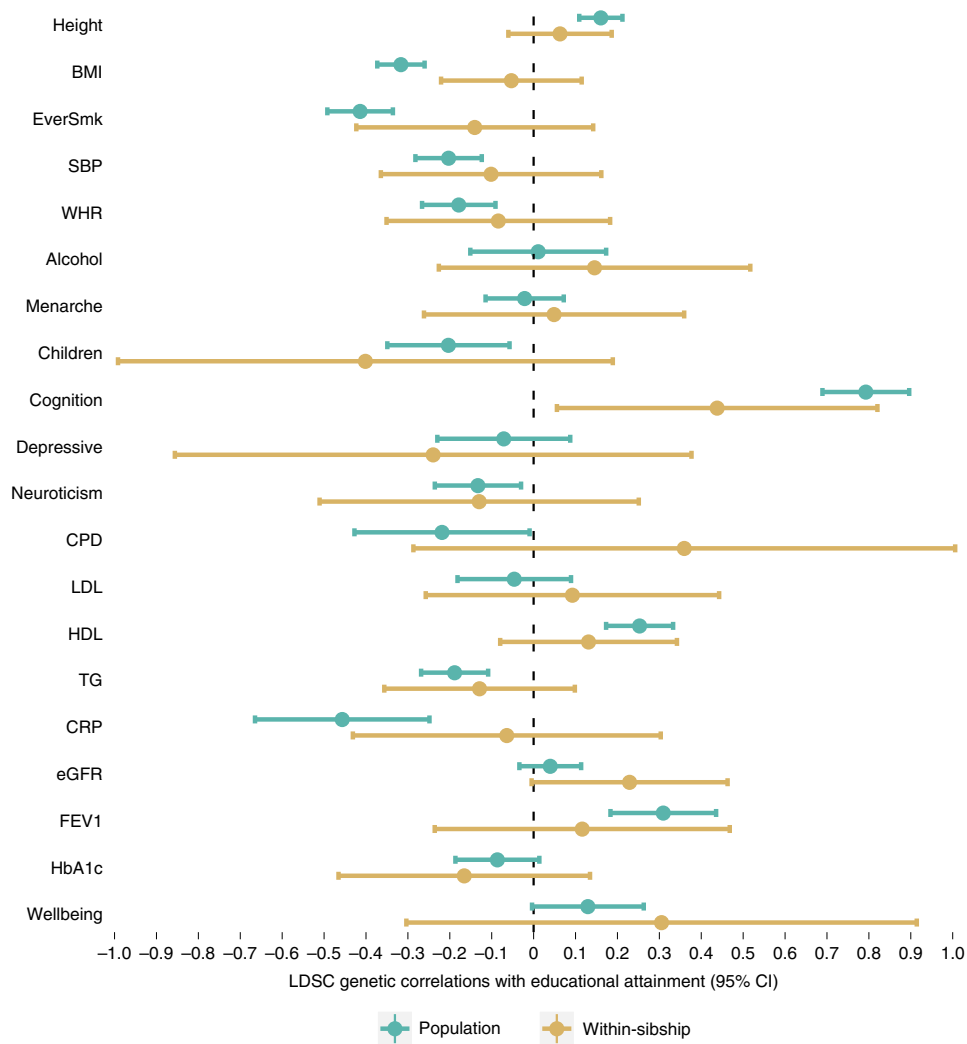
Fig. 6 | LDSC r_g estimates between educational attainment and 20 phenotypes using population and within-sibship meta-analysis data with corresponding 95% CIs. The number of individuals contributing to the educational attainment GWAS was n = 128,777 with sample sizes for outcomes ranging from n = 149,174 for height to n = 27,638 for cognitive ability. BMI, body mass index; Education, educational attainment; EverSmk, ever smoking; SBP, systolic blood pressure; WHR, waist-hip ratio; Alcohol, weekly alcohol consumption; Menarche, age at menarche; AFB, age at first birth; Children, number of biological children; Menopause, age at menopause; Cognition, cognitive ability; Depressive, depressive symptoms; CPD, cigarettes per day; LDL, LDL cholesterol; HDL, HDL cholesterol; TG, triglycerides; CRP, C-reactive protein; eGFR, estimated glomerular filtration rate; FEV1, forced expiratory volume; HbA1c, Haemoglobin A1C. Further information on the sample sizes of each phenotype is contained in Supplementary Table 2.
