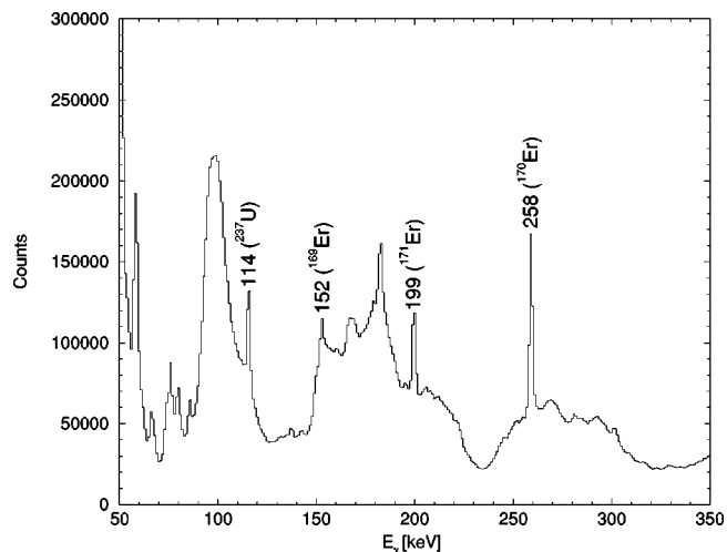
FIG. 2. Delayed \gamma -ray spectrum for the reaction between ^{170}\text{Er} and ^{238}\text{U} at E_{\text{c.m.}} = 566 MeV. The peaks labeled by their \gamma -ray energies are the known transitions from the nucleus specified under parentheses. No Doppler-shift correction was applied to these spectra.
