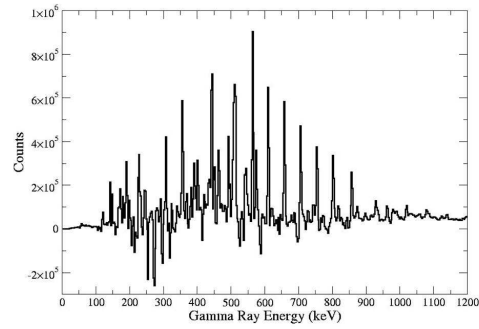
Fig. 5. Gamma-gamma gated gamma-ray coincidence spectrum for TSD Band 1 in ^{167}\text{Lu} . Transitions belonging to TSD band 1 are clearly visible as are transitions connecting lower-lying normal-deformed states. The spectrum is obtained by summing all pairs of gates on TSD Band 1 transitions from 505 to 1192 keV.
