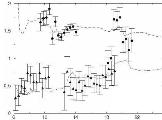
Fig. 1. The first test of the surrogate ratio method, adapted from [7]. The top set of data (circles) is the ratio of \frac{N({}^{238}\text{U}(d,pf))}{N({}^{236}\text{U}(d,pf))} , surrogate for \frac{\sigma[{}^{238}\text{U}](n,f)}{\sigma[{}^{236}\text{U}](n,f)} and is compared to the accepted value for the ratio extracted from the databases (dashed line). The lower data (triangles), the ratio of \frac{N({}^{238}\text{U}(d,df))}{N({}^{236}\text{U}(d,d'f))} , is surrogate for the unknown \frac{\sigma[{}^{238}\text{U}](n,f)}{\sigma[{}^{236}\text{U}](n,f)} ratio of cross sections. The x -axis shows the excitation energy in MeV.
