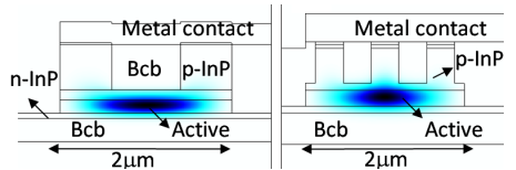
Figure 2. Mode profile in two optimized designs.
