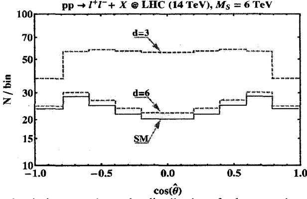
FIGURE 3. Bin integrated angular distributions for lepton pair production at LHC in the SM and ADD scenario integrated over lepton pair invariant mass in the range between 1500 GeV and 2000 GeV at M_S = 6 TeV and d=3, 6 .
