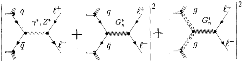
FIGURE 1. Feynman diagrams for dilepton production at leading order in ADD model.
