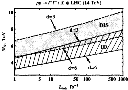
FIGURE 4. Discovery (gray band) and identification (hatched band) reaches on M_S (in TeV) at 95 % CL as a function of integrated luminosity L_{\text{int}} for different number of extra dimensions ( d = 3 - 6 ) at the LHC with 14 TeV.
