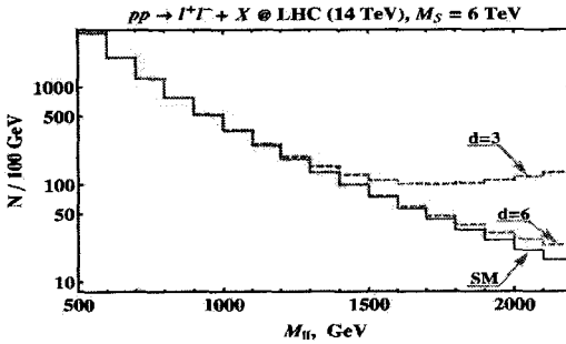
FIGURE 2. Effects of extra dimensions on the dilepton mass spectrum at LHC with s = 14 TeV and integrated luminosity 100 \text{ fb}^{-1} . Histograms show the spectrum in the SM as well as in ADD scenario with cutoff M_S = 6 TeV and different number of extra dimensions ( d = 3, 6 ) at LHC with s = 14 TeV and integrated luminosity 100 \text{ fb}^{-1} .
