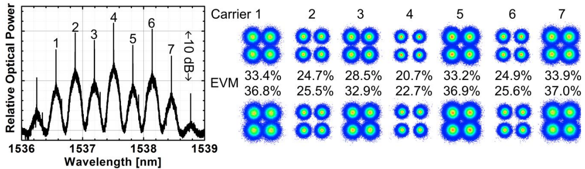
Fig. 3: Data transmission results: Data transmission of 784 Gbit/s using QPSK signals on 7 carriers generated by an integrated SOH comb source. Comb spectrum (left) and constellation diagrams for all channels and both polarization are depicted along with measured EVM values. BER below hard-decision threshold are achieved for all signals.
