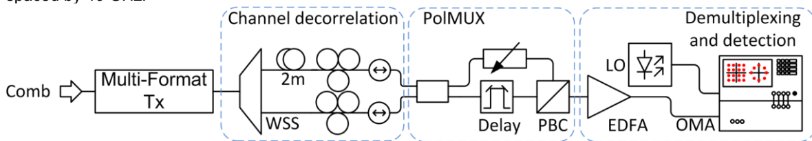
Fig. 2: Data transmission setup: Each comb line is modulated with a 28 GBd QPSK signal. Even and odd channels are separated with a wavelength-selective switch (WSS) to decorrelate neighboring channels. Both data streams are merged and are polarization multiplexed (PolMUX). After amplification, the channels are demultiplexed and detected by an optical modulation analyzer (OMA) and a tunable laser acting as a local oscillator (LO).
