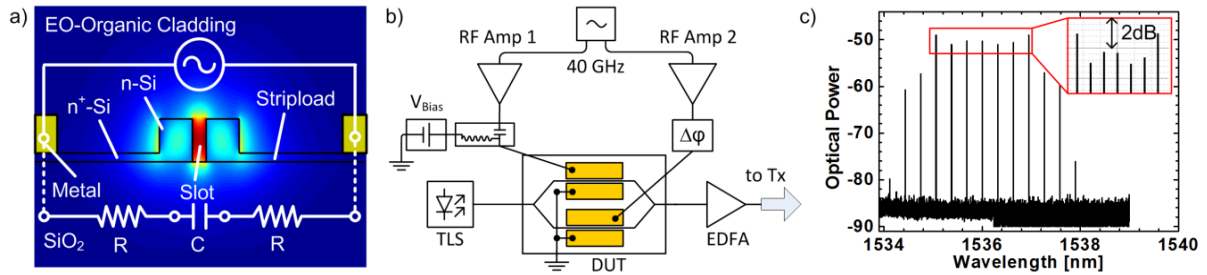
Fig. 1: a) Schematic and simulated optical mode of a silicon-organic hybrid (SOH) phase-modulator. The two rails of a silicon slot waveguide are electrically connected to metal electrodes by 60 nm high n -doped silicon slabs. The waveguide is covered by an electro-optic cladding material (DLD164), which entirely fills the slot. b) Integrated frequency comb generator: A tunable laser source (TLS) is coupled to a dual-drive SOH Mach-Zehnder modulator (MZM) via grating couplers. The arms are driven by two sinusoidal 40 GHz signals. Flat combs are obtained by carefully adjusting the signal powers and phases along with the bias voltage V_{\text{Bias}} . Fiber-chip coupling losses are compensated by an erbium-doped fiber amplifier (EDFA). c) Flat-top spectrum obtained for electrical drive powers of 28 dBm and 23 dBm, showing 7 lines within 2 dB flatness. The lines are spaced by 40 GHz.
