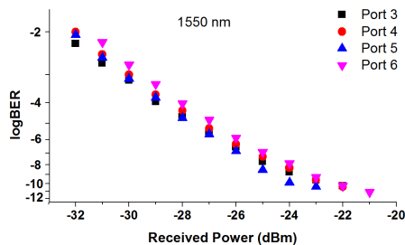
Figure 3b BER vs. received power, \lambda=1550 nm
