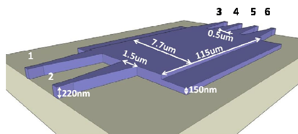
Figure 1 Schematic of the 2x4 MMI
