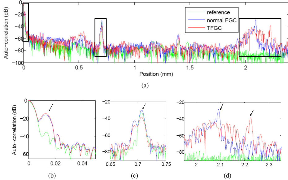
Fig. 3. 3(a) : Autocorrelation of reflections from three test structures: a normal focusing grating coupler (FGC), a tilted focusing grating coupler (TFGC), and an empty area (reference). Three important reflections are shown: 3(b) reflections from the input grating coupler, 3(c) reflections from the chip backside, and 3(d) reflections from the output grating couplers.
