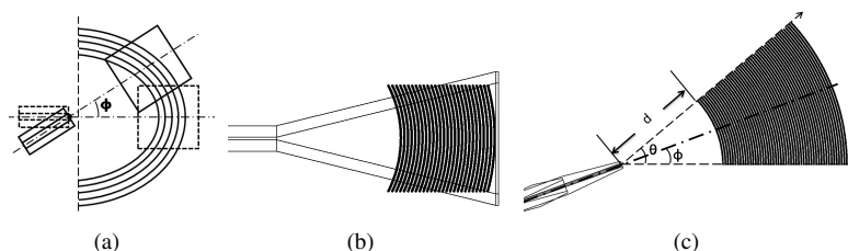
Fig. 1. 1(a): Schematic illustration of the ellipses used in focusing grating couplers (FGCs) on SOI. The dashed box shows the part used by a normal FGC. In our proposal, the grating in the box with a nonzero azimuthal angle \phi is used. 1(b): a normal FGC. 1(c): a TFGC with an azimuthal angle \phi = 20^\circ and an opening angle of \theta = 40^\circ .
