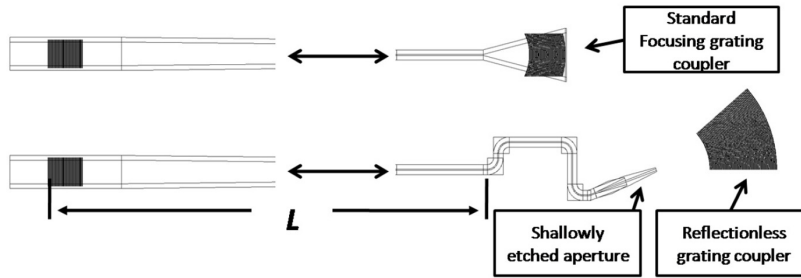
Fig. 2. Two different structures were measured: a normal FGC and a TFGC. Laser signals were sent from the left side through the standard grating couplers, and connected to the test grating couplers through a straight taper with a length of around 2 mm.
