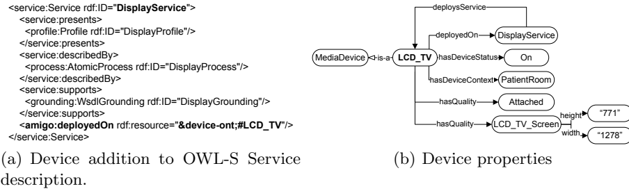
Fig. 2. Service deployment on context-rich devices.
