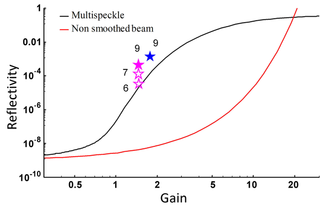
Figure 9. Curves of the growth of SRS reflectivity obtained from a multispeckle model (black) and a non-smoothed beam (red) as a function of the Rosenbluth gain calculated for the nominal laser intensity. Magenta and blue stars represent experimental results in shots without and with the driver beams, respectively, where the gain has been calculated considering the single-beam intensity. Empty stars represent shots with a smaller number of beams, as indicated by numbers 6, 7 and 9. The relative uncertainty of the reflectivity values due to the calibration procedure is around 30%, which is as large as the star size.
