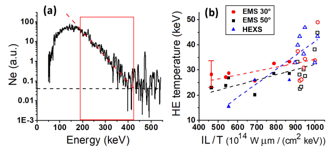
Figure 7. (a) Typical HE spectrum obtained by the EMSs, where the red rectangle shows the fitting region and the black dashed line is the background level. (b) Values of HE temperature obtained by the EMSs at 50° (black squares) and at 30° (red circles) and by the HEXS (blue triangles) versus the I_{ov}L/T parameter. Solid and empty symbols indicate the shots without and with the driver beams, respectively. The relative uncertainty is 20% for all datasets, indicated as an example by the error bar on the left. The dashed lines represent the linear fitting for the complete sets of EMSs at 30°, EMSs at 50° and HEXS data.
