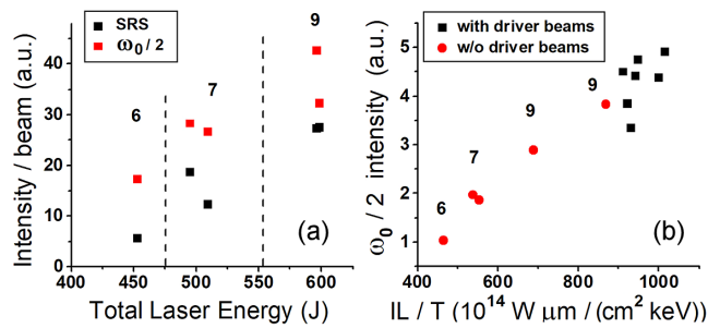
Figure 6. (a) SRS and \omega_0/2 intensities normalized by the number of beams versus the total laser energy. Measurements here refer to shots without the driver beams. Labels 6, 7 and 9 indicate the number of laser beams switched on in the shots. (b) Growth of \omega_0/2 intensity versus the parameter I_{ov}L/T .
