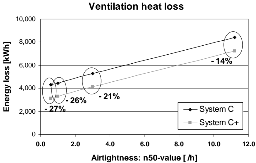
7 8 Figure 8: Energy loss - airtightness
