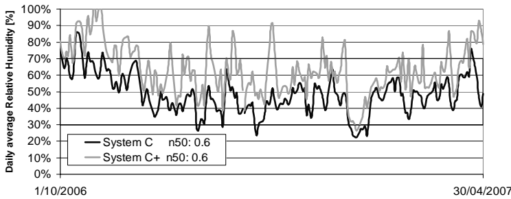
Figure 6 & 7: Relative Humidity in Bedroom 1
