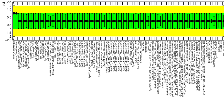
(a) Asimov
