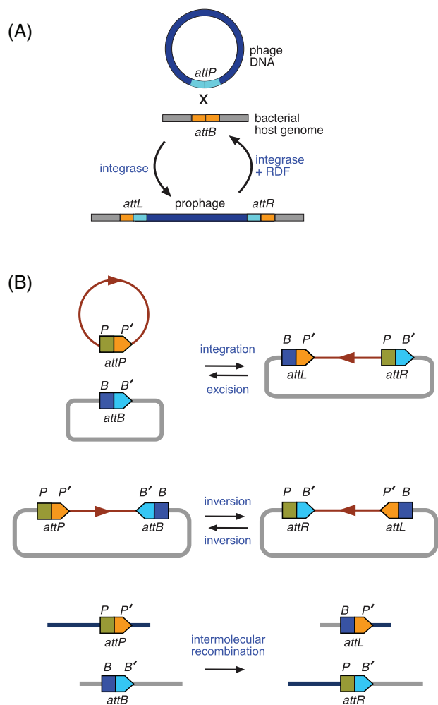
FIGURE 1 Site-specific recombination by LSIs, and outcomes of recombination events. (A) Phage integration into bacterial host genome. In their natural context, LSIs recombine an attP site in the phage DNA and an attB site in the genome of the bacterial host, resulting in integration of the phage DNA as a prophage. This unidirectional reaction generates two new recombination sites: attL (formed from the left end of attB and right end of attP ), and attR (formed the left end of attP and right end of attB ). In the reverse reaction, a second host protein termed the RDF binds to the LSI and changes its specificity to recombine attR and attL , thereby reforming attB and attP . Adapted from Olorunniji et al. [26] (B) Outcomes of site-specific recombination by LSIs. Intermolecular recombination between att sites results in integration of a circular DNA molecule into a corresponding genomic locus. In the reverse reaction, intramolecular recombination of compatible att sites arranged in “head to tail” (or “direct repeat”) orientation results in an excision (resolution) outcome. In contrast, when sites are in “head to head” (or “inverted repeat”) orientation, the outcome of the recombination event is inversion, that is, “flipping” of the DNA segment flanked by the recombining att sites. Finally, intermolecular recombination involving linear DNA molecules generates two different linear recombinant molecules. The functional annotation of attP (P–P′) and attB (B–B′) sites are shown to illustrate the site orientations in the recombinant attR (P–B′) and attL (B–P′) sites, respectively. Adapted from Olorunniji et al. [3] LSI, large serine integrase; RDF, recombination directionality factor.
