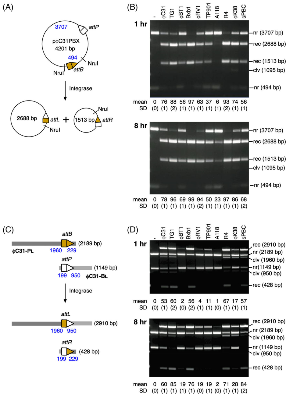
FIGURE 2 in vitro activities of attP x attB recombination activities of serine integrases. (A) Scheme illustrating the in vitro intramolecular recombination assay (substrate plasmid pφC31PBX for φC31 integrase is shown; other integrase substrates are similar). The plasmid substrates are named after the large serine integrase (LSI) (φC31) and the att sites that will recombine (PBX; attP x attB resolution reaction). (B) Intramolecular recombination of attP x attB plasmid substrates by selected serine integrases (φC31, TG1, φBT1, Bxb1, φRV1, TP901, A118, φR4, φK38, and SPBC). Reactions were incubated for 1 or 8 h in the reaction buffer described in Section 2. Reaction products were digested with the restriction endonuclease NruI prior to 1.2% agarose gel electrophoresis. The final integrase concentrations were 800 nM in all cases. Top panel: 1-h reactions; Bottom panel: 8-h reactions. The bands on the gel are labeled nr (non-recombinant, i.e., substrate), rec (recombination product), clv (cleavage product). The sizes of the products of the recombination reactions are shown next to each band on the gel image. The mean extent of recombination and standard deviation (%) from quantitation of triplicate experiments are given below each lane. (C) Scheme illustrating the in vitro intermolecular recombination assay using linear DNA substrates (φC31-PL and φC31-BL for φC31 integrase is shown; other integrase substrates are similar). The sizes of the linear DNA substrates and the position of the att sites on them are designed to allow clear separation and identification of the reaction substrates and products using agarose gel electrophoresis. The sizes of the products of the recombination reactions are shown next to each band on the gel image. (D) Intermolecular recombination of attP x attB linear substrates by selected serine integrases. Reactions were incubated for 1 or 8 h in the reaction buffer described in Section 2. Reaction products were separated by 1.2% agarose gel electrophoresis. The final integrase concentration was 800 nM in all cases. Top panel: 1-h reactions; Bottom panel: 8-h reactions. The bands on the gel are labeled nr (non-recombinant, i.e., substrate), rec (recombination product), clv (cleavage product). The mean extent of recombination and standard deviation (%) from quantitation of triplicate experiments are given below each lane.
