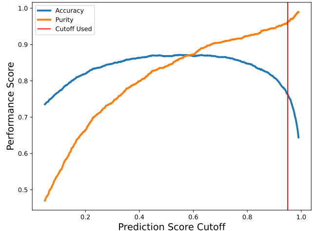
Figure 4. A measure of accuracy and purity against prediction score. The accuracy (in blue) is a direct measure of the number of sources Zoobot correctly predicted vs the total number of predictions made. The measure of purity (in orange) is the the number of predictions Zoobot correctly made vs the total number of predictions for an interacting galaxy. The cutoff score (in red) shows the point above which we would define an interacting galaxy and below which we would not. At this point, the accuracy appears lower due to Zoobot making many false negative predictions while successfully making true negative predictions. This is confirmed by the maximisation of purity. Due to the number of sources Zoobot is predicting over, the size of the catalogue will exceed any previous catalogues. Therefore, we use this very conservative cutoff to maximise purity over the completeness of our catalogue. These measures can also be shown with the F1 score. Figure 15 shows this change with prediction cutoff in the Appendix.
