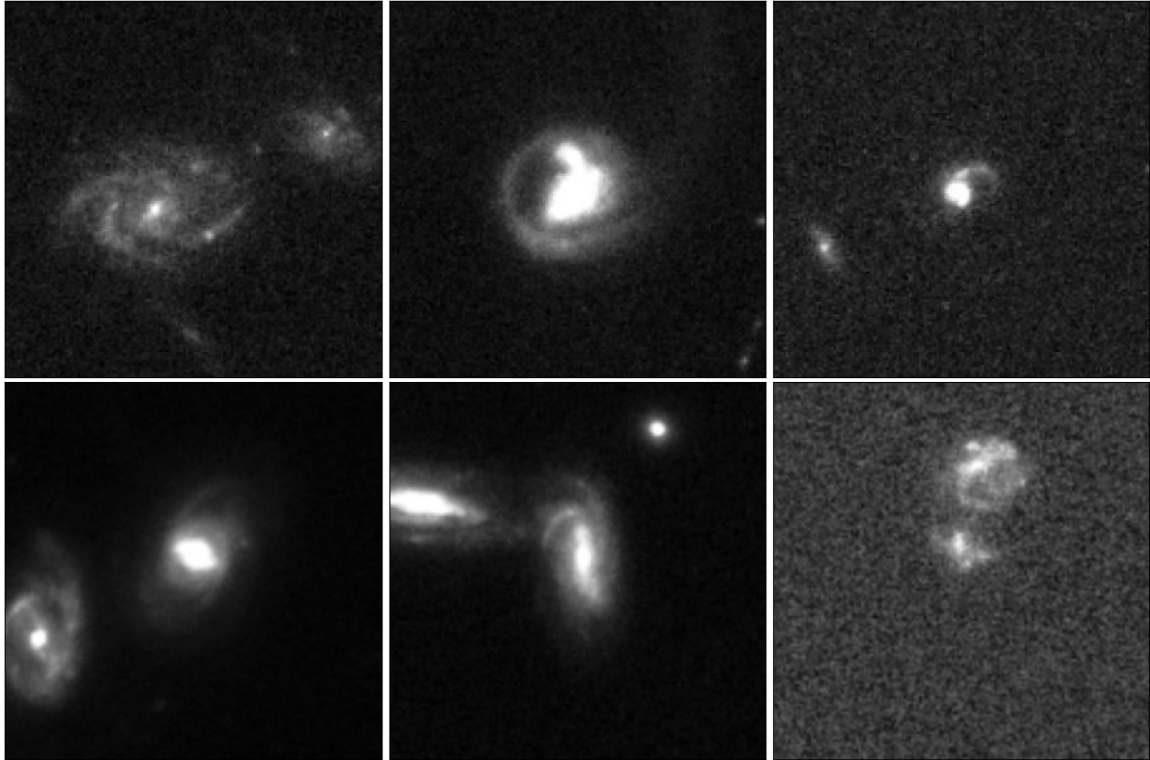
Figure 1. Example images of the labelled interacting galaxy systems used to train Zoobot . Each galaxy had a weighted vote fraction \geq 0.75 in Galaxy Zoo. Top Row : Three examples from the Galaxy Zoo: Hubble project of the training set. Bottom Row : Three examples from the other Galaxy Zoo projects. These are, from right to left, Galaxy Zoo 2, Galaxy Zoo CANDELS and Galaxy Zoo DECaLS. The priority with this training set was that the interactors had clear tidal features and disruption so Zoobot would learn to highly weight them and not misclassify close pairs.
