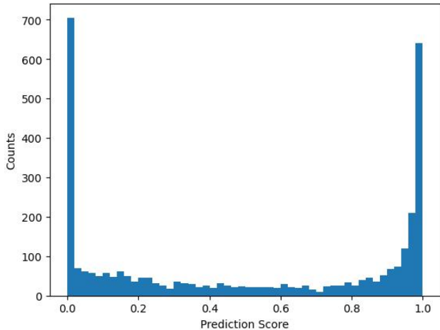
Figure 3. The distribution of prediction scores given to our validation set of 3,270 labelled sources set aside by Zoobot in training. These were split into 1,648 non-interacting sources and 1,622 interacting sources. As can be seen from the distribution, our model is often confident when a source does or does not contain an interacting galaxy by the strong bimodality. This is likely due to the very stringent vote weightings used when selecting the training set. Using this distribution, we decide the prediction score to use as a cutoff to give us our final binary classification: interacting galaxy or not.
