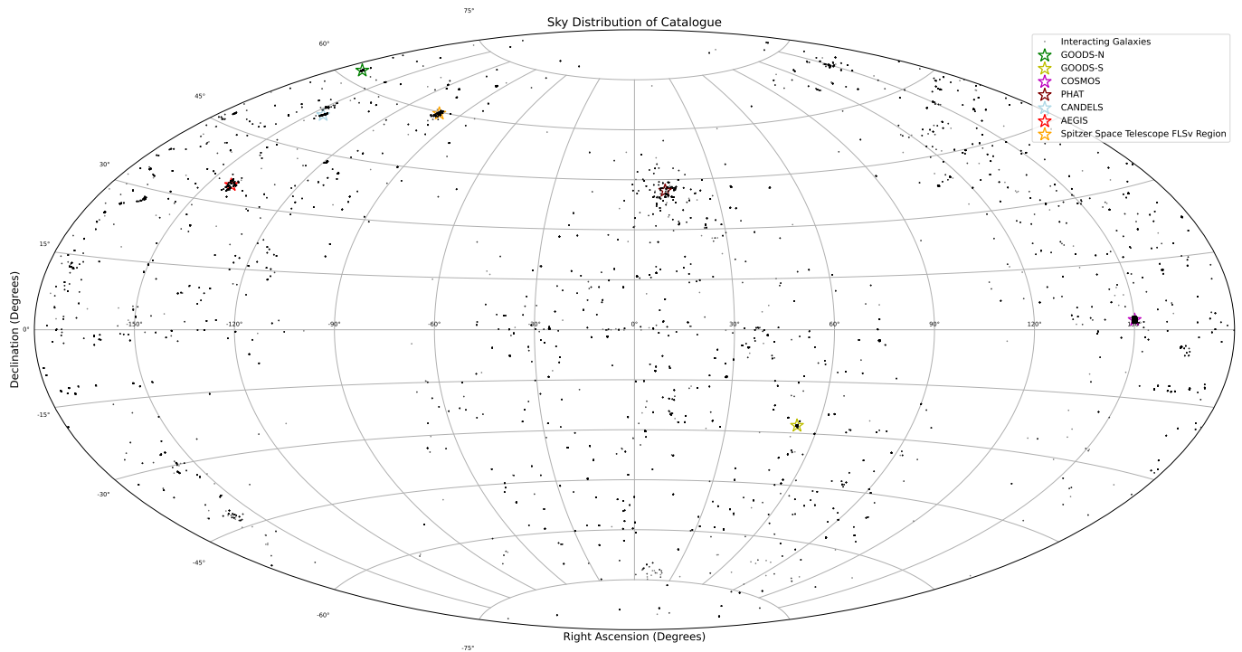
Figure 10. Sky Distribution of our catalogue, with marked positions of well known deep surveys conducted by HST . HST is able to observe almost the entire sky and therefore the interacting galaxies are scattered throughout. Large clusters of sources are found in the locations of surveys. This shows that often our sources are in the background of larger surveys and observations.
