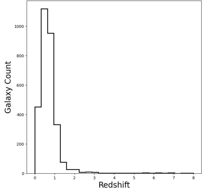
Figure 11. The redshift distribution of a subsample of our catalogue. Of the 7,583 referenced systems, 3,037 of them had redshift measurements in the NED, MAST or Simbad. This redshift distribution shows that our model confidently predicted interacting systems primarily for z < 1 systems. This was anticipated, as the model was primarily trained on systems at these redshifts. There are fifteen sources with a reported z > 5 .
