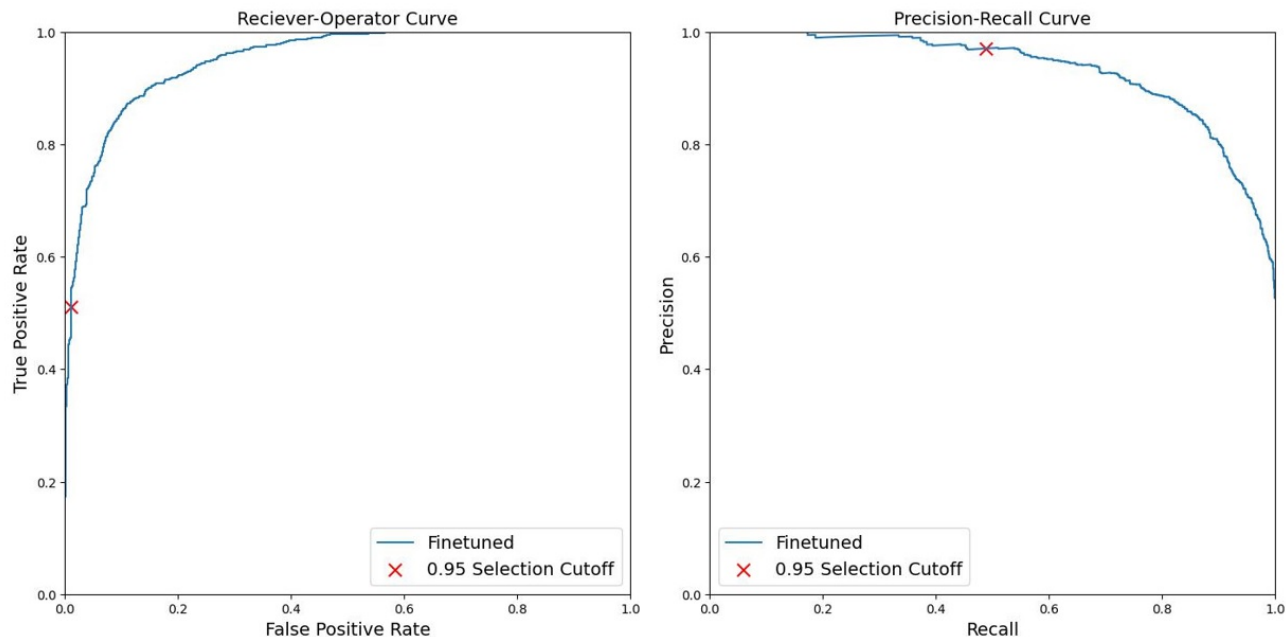
Figure 14. The Receiver-Operator and Precision-Recall Curve for the Zoobot model that was used to explore the Hubble archives. The blue curves are the measured curves. These curves measure the relevant rates or characteristics based on the changing cutoff applied to how Zoobot defines an interacting galaxy. The red crosses are where the prediction score cutoff is for this work. We can see in the Receiver-Operator Curve that the prediction score cutoff we use would have an incredibly low false positive rate, while it would be misclassifying \approx 50\% of interacting galaxies. This is also shown in the precision recall curve where our recall is \approx 50\% .
