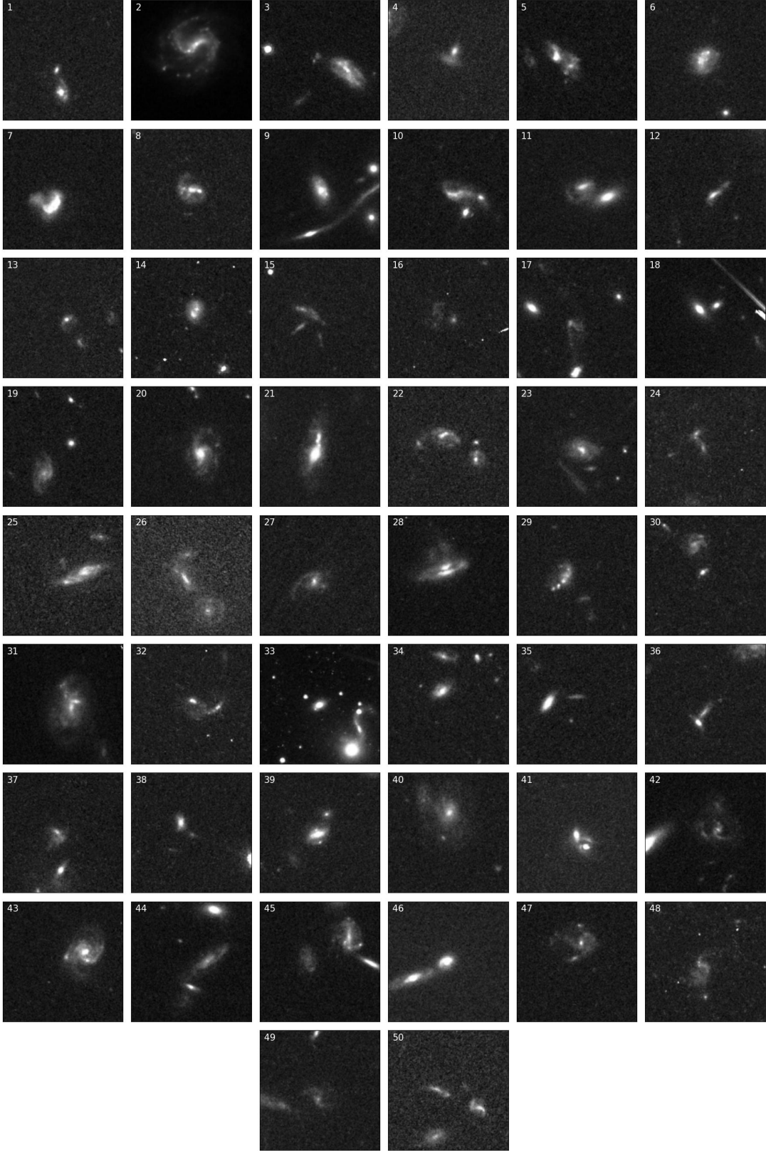
Figure 9. An example of 50 of the final interacting systems found with Zoobot. These were selected randomly from the de-duplicated and de-contaminated 21,926 sources. Each of these examples have extended tidal features and distortion. Not all of the final interacting systems have two galaxies within them (for example, image 2), but are clearly very disturbed by a tidal event. These were kept in as they would form a large part of the interacting galaxy population and would be flagged as disturbed or interacting in Galaxy Zoo. Each of these images is a 1-colour image using the F814W HST filter.
