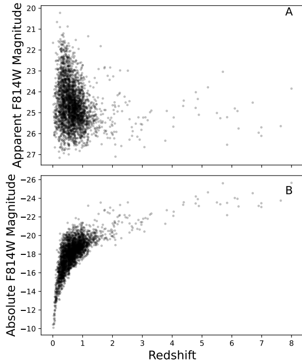
Figure 12. The distribution of redshift with magnitude for all sources with available data. This shows the parameter space we are sampling in this catalogue. Panel A shows that the majority of our sources are dim, background sources at low redshift. Panel B shows the faintest objects we find are at the limiting magnitudes of the different surveys this data is from.
