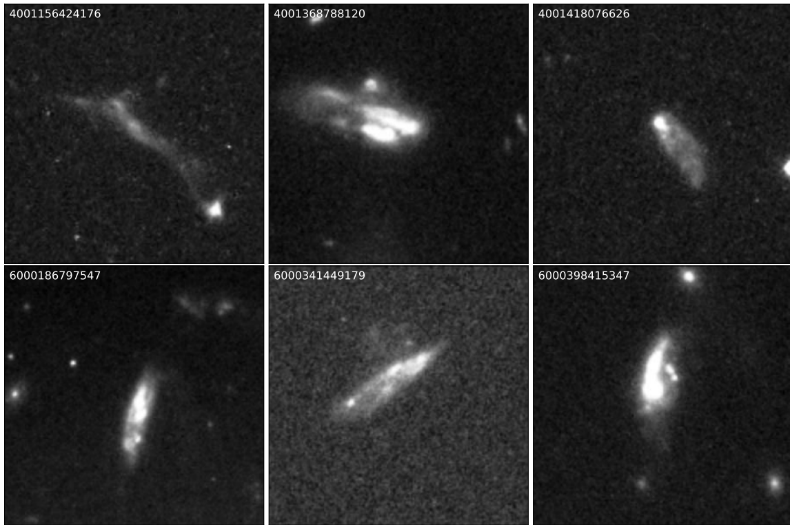
Figure 17. The six unknown systems found in this work. These have no reference in Simbad or in NED, and their morphology could not be classified by the authors. Investigation into these six objects are presented to the community, with the authors hoping that future work and investigation of them can be conducted by them.
