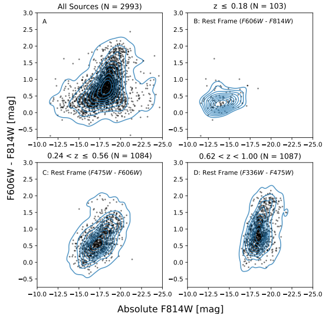
Figure 13. The colour-magnitude distribution of sources with a redshift measurement associated. Panel A shows the distribution of all galaxies, without controlling for redshift or dust extinction. The remaining panels then split these sources into distinct redshift bins where the F606W and F814W filters are observing in different rest frames. Panel B shows the colour-magnitude distribution in the local universe, where the rest frame observations are F606W and F814W flux. This bin reveals a blue population. Panel C shows the redshift bin where at 50% - 100% of observed F606W and F814W flux is rest frame F475W and F606W flux. This bin reveals a larger distribution of interacting galaxies, with a dominating population of blue systems and a minor population of red systems. Panel D shows the redshift bin where 50% to 100% of observed F606W and F814W flux is rest frame F336W and F475W flux. These filter bands are very sensitive to star formation, and reveal a broad distribution in colour of red and blue systems.
