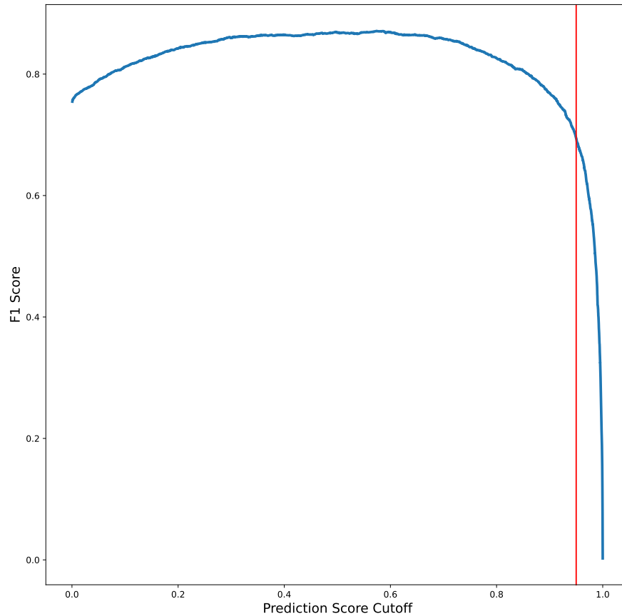
Figure 15. The F1 score found during the diagnostics of the model used in this work. The F1 score is a measure combining the measure of accuracy and purity into one metric. The cutoff we use is at the point where the F1 score begins to rapidly decline. This point is shown by the red vertical line.
