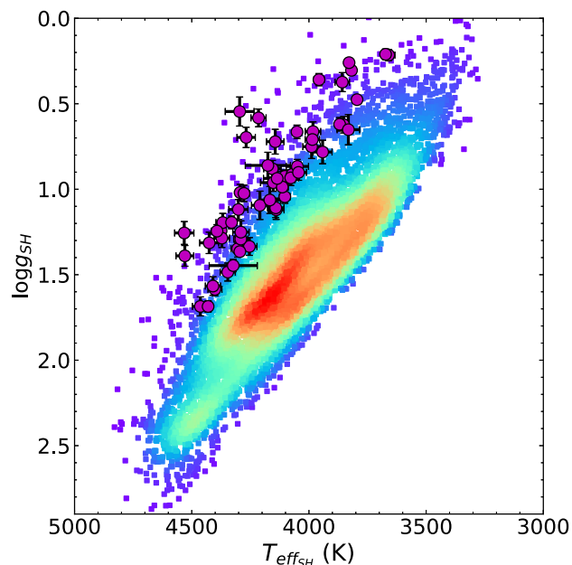
Figure 3. Kiel diagram of the 58 sample bulge stars (purple circles). In the background, we show the full reduced proper-motion sample of Queiroz et al. (2021).
