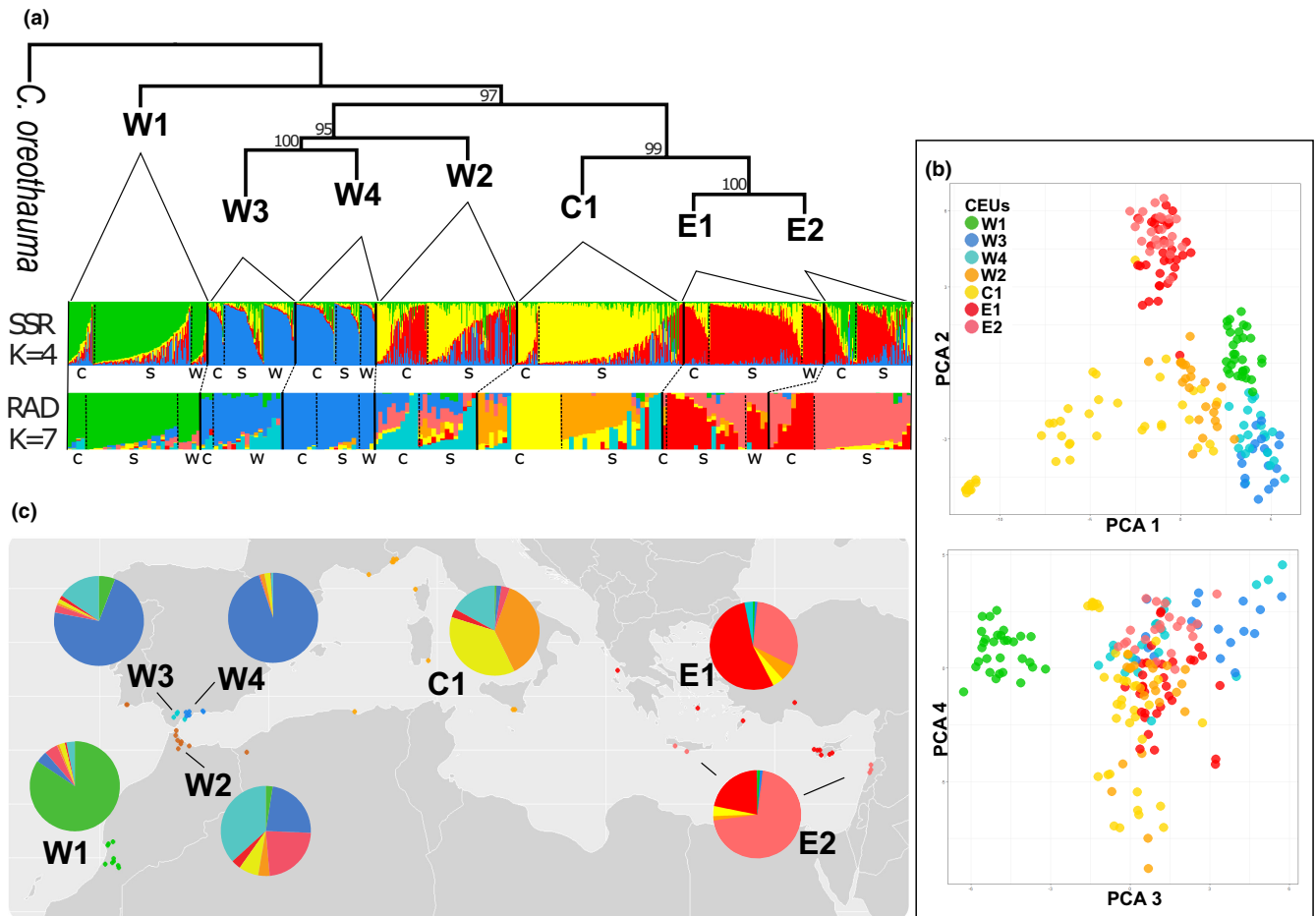
FIGURE 4 Population genetic structure of the carob tree. (a) SVDQUARTETS tree of seven genetically and geographically homogeneous groups (CEUs) based on RADseq markers. Genetic admixture plots are based on four ancestral populations for SSR markers (1019 genotypes, 17 loci) and on seven ancestral populations for RADseq markers (190 genotypes, 3557 neutral unlinked SNPs). Within CEUs, genotypes were organized by habitats and according to their admixture coefficient (c = cultivated, s = seminatural and w = wild). (b) PCA scatterplots of RADseq genotypes (accumulated variance of the first four components = 15.2%). (c) Map of genetic admixture based on RADseq markers
