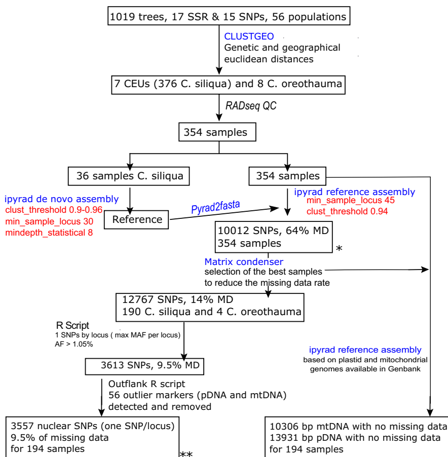
FIGURE 1 Bioinformatic pipeline used to call and filter SNPs from RADseq data for the carob tree. Asterisks (* and **) correspond to the two data sets of Table 1. Raw data and filtered vcf files (* and **) are available (see Data Availability statement)
