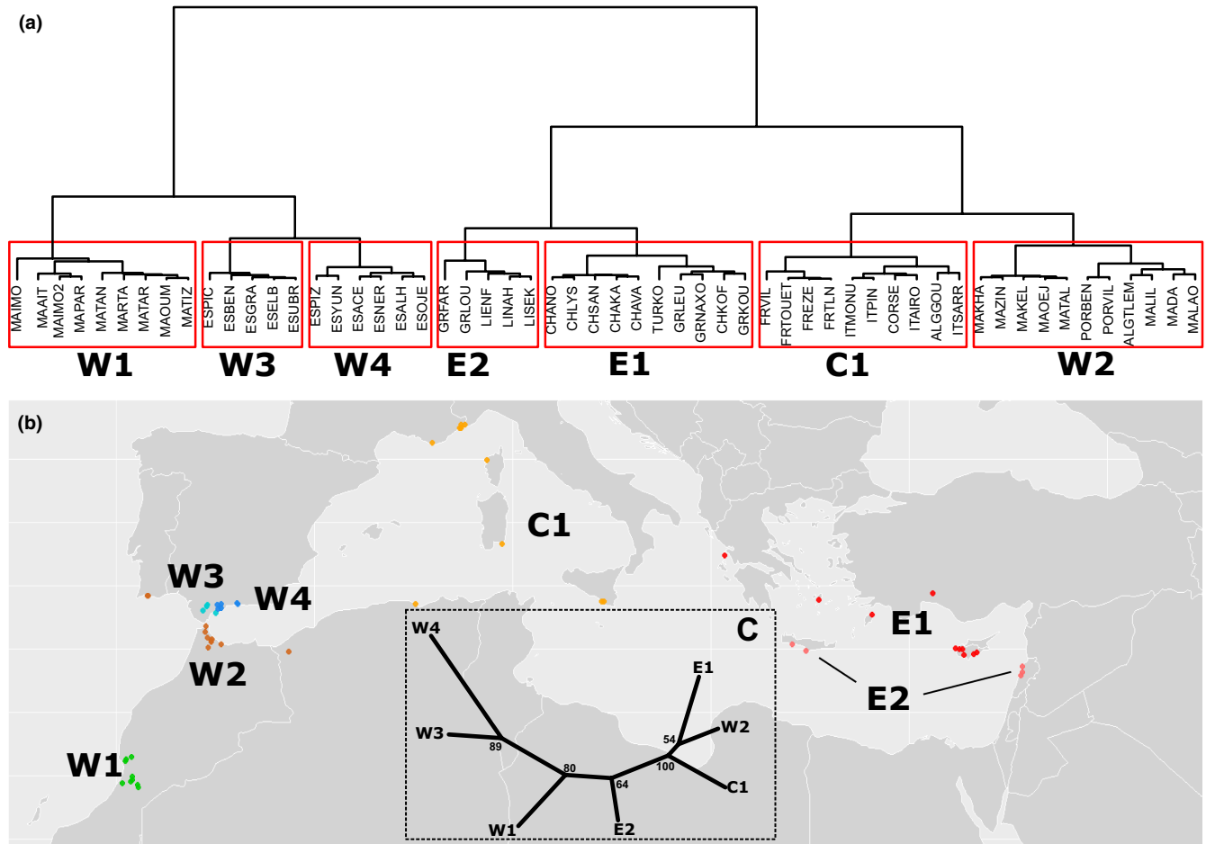
FIGURE 2 Identification of carob evolutionary units (CEUs) using the ClustGeo method, which considers Euclidean genetic and geographical distances. The analysis used 1,019 genotypes from 56 localities based on 17 SSRs and 15 SNP markers from microsatellite loci. The Ward dendrogram of 56 carob populations with a partition into K = 7 clusters (a) was obtained with a normalized proportion \alpha of explained inertia of 0.2 for the geographical distance and 0.8 for the genetic distance. The seven clusters, or CEUs, are mapped (b) and a neighbour-joining tree (c) shows pairwise genetic differentiation (Gst SSR markers) among the seven clusters. W1 = southwest Morocco, W2 = mainly north Morocco but also west Algeria and Portugal, W3 = west Andalusia, W4 = East part of Andalusia, C1 = France, Italy and Algeria, E1 = Greece, Turkey and Cyprus, E2 = Lebanon and Crete (Greece); see details in Table 1
