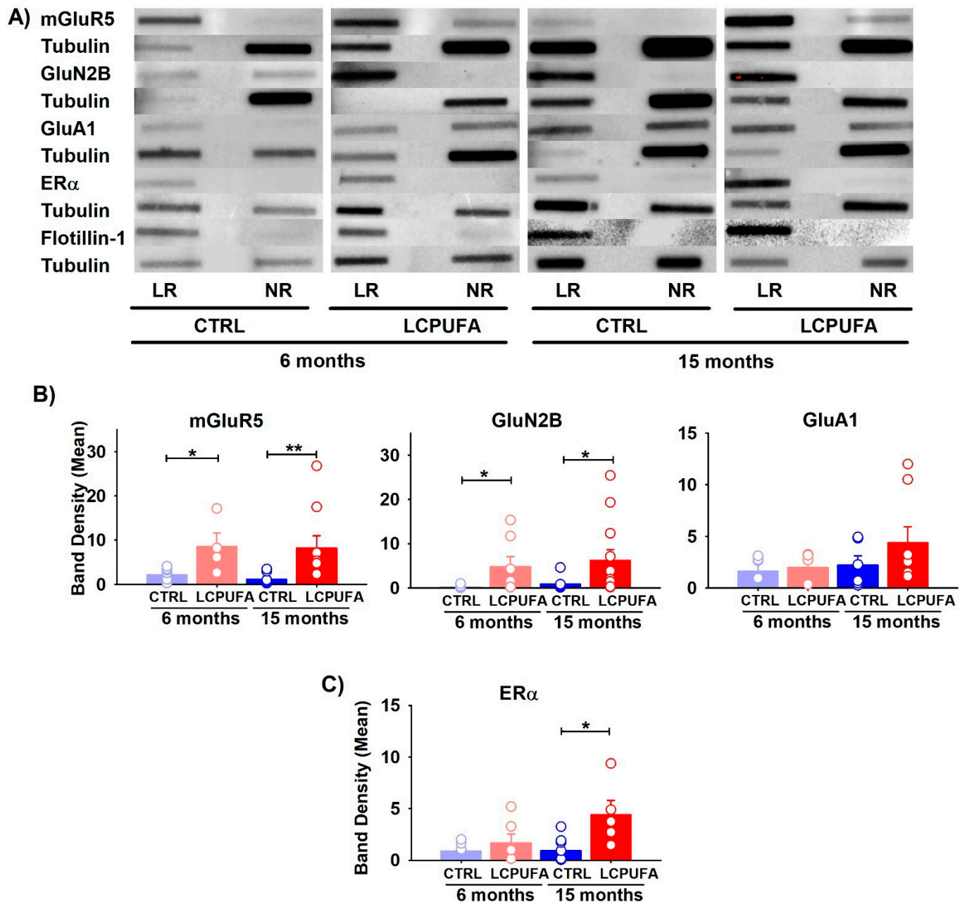
Figure 2. Differential expression of receptors in lipid raft fractions of the hippocampus. (A) Representative bands obtained by slot blot technique are shown for each condition. Tubulin expression was used as the charge control and flotillin-1 as the control from lipid raft fractions. In all cases, lipid raft fraction (LR) and non-raft fraction (NR) are shown. (B) Effect of age and diet on glutamatergic receptors expression. (C) Effect of age and diet on ER \alpha expression. Bars represent the means of band density \pm SEM of 4–12 mice per group (bands: mGluR5 6 m n = 7 and 15 m n = 9 ; GluN2B 6 m n = 8 and 15 m n = 12 ; GluA1 6 m n = 5 and 15 m n = 8 ; ER \alpha 6 m n = 6 and 15 m n = 7 ). Circles represent each individual measurement. Data were analyzed by a 2-way ANOVA (diet, age) and Tukey's post hoc test (* p < 0.05 , ** p < 0.01 ). Data analysis was performed after normalization of the normalization of band intensity relative to tubulin.
