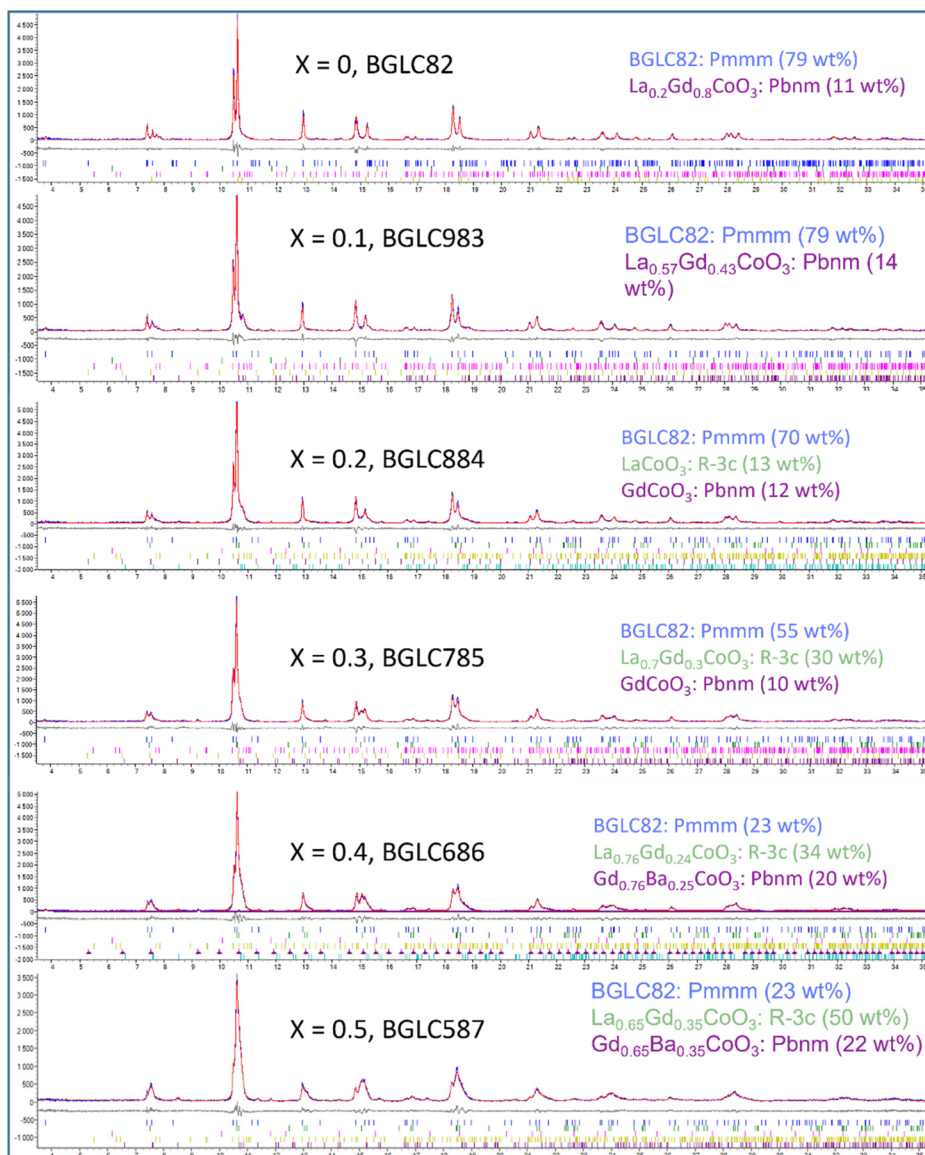
Fig. 2 SR-PXD rietveld refinements (red line) of BGLC ( x = 0 – 0.5 , y = 0.2 ). Minority phases \text{Co}_3\text{O}_4 , \text{Gd}_2\text{O}_3 and \text{BaCO}_3 are refined, but omitted in the figure legends.
