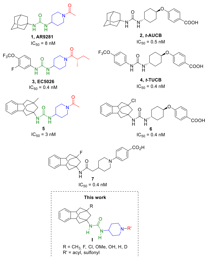
Figure 2. Structures and IC 50 values in the human sEH of AR9281, 1, t -AUCB, 2, EC5026, 3, t -TUCB, 4, 5, 6, and 7 and general structure I, of the new derivatives reported on this work.
