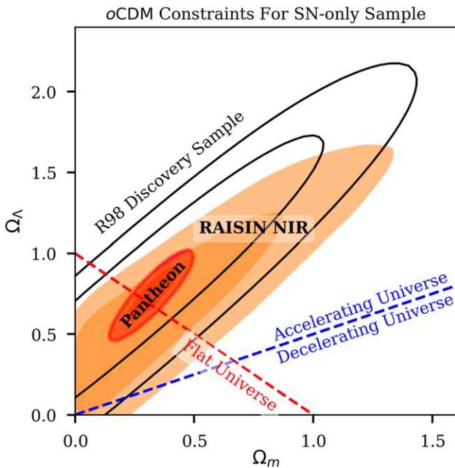
Figure 11. Cosmological parameter measurements from \omega CDM (a CDM model allowing nonzero curvature) with SNe alone. Open contours show the Riess et al. (1998) discovery sample, red contours show the Pantheon constraints from Scolnic et al. (2018), and the results from RAISIN SNe are in orange. All contours show the 68% and 95% confidence intervals.
