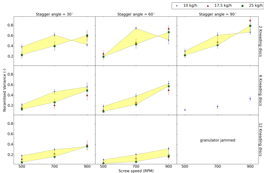
Figure 4.7: Normalised variance \sigma_{\theta}^2 and the standard deviation based on the experimental RTD profile at various material throughputs (10-25 kg/h), number of kneading discs (2, 6, 12), stagger angle (30-90°) and different screw speeds (500-900 rpm)
