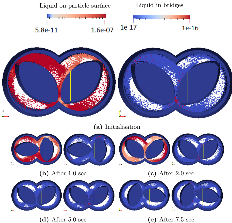
Figure 10.7: Changes on volume of liquid on particle surface (left side snapshot in each sub-plot) and liquid in bridges (right side snapshot in each sub-plot) when two kneading discs were co-rotating at 100 rpm and at a Q_{lod} of 7.5 \times 10^{-4} .
