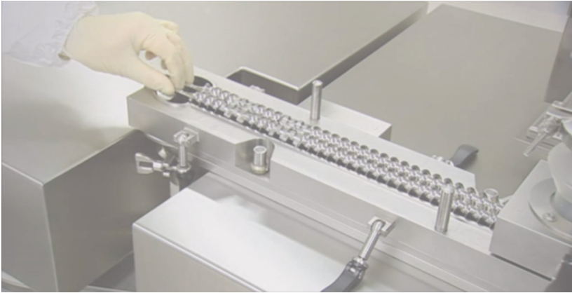
Figure 3.4: Twin-screw granulator from lab-scale continuous processing equipment ConsiGma TM -1 with the granulator barrel that can be opened.
