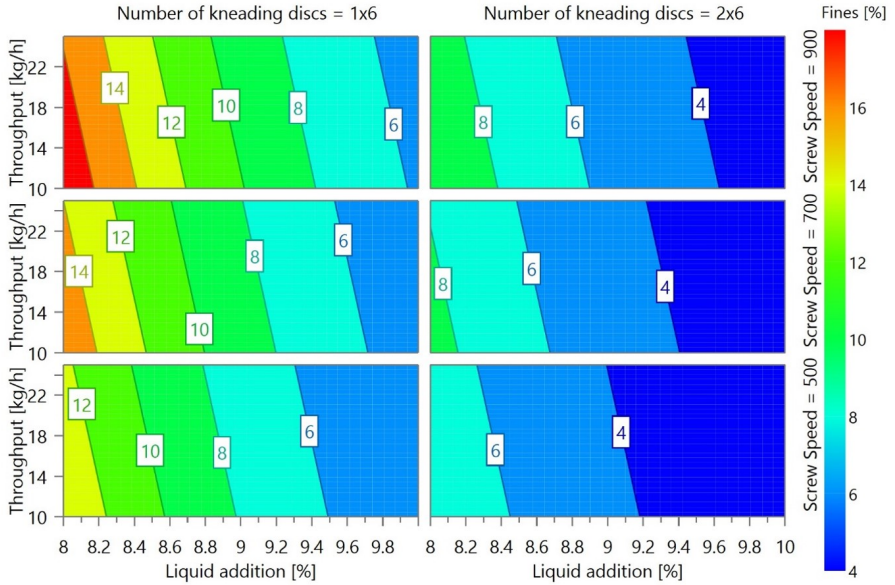
Figure 9.4: Change in fines fraction ( <150 \mu\text{m} ) in the granules produced at different screw speeds (500, 700, 900 rpm), material throughputs (10-25 kg/h), number of kneading discs ( 1\times 6 , 2\times 6 ) and stagger angle ( 60^\circ ).
