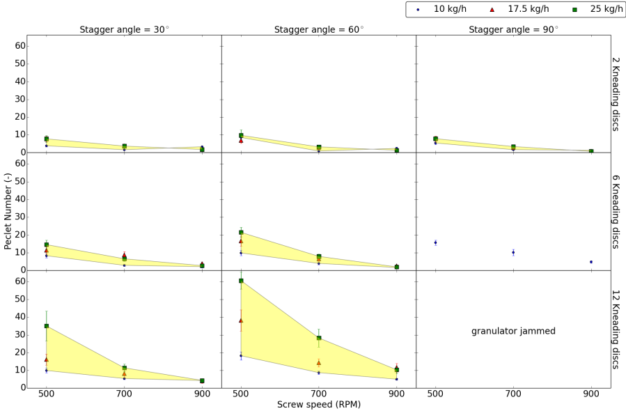
Figure 4.8: Peclet number (Pe) and the standard deviation based on the experimental RTD profile at various material throughputs (10-25 kg/h), number of kneading discs (2, 6, 12), stagger angle ( 30^\circ - 90^\circ ) and different screw speeds (500-900 rpm)
