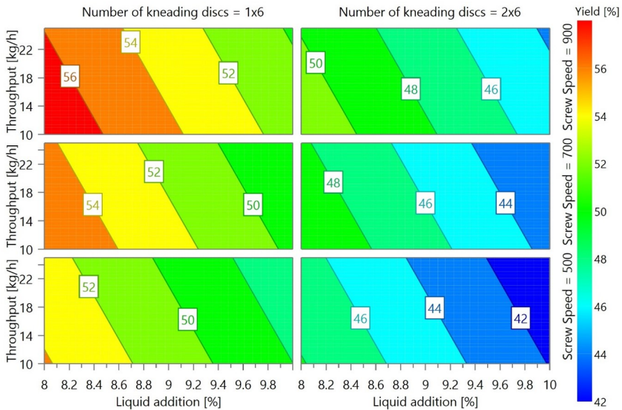
Figure 9.5: Change in yield fraction (150 - 1400 \mu\text{m} ) in the granules produced at different screw speeds (500, 700, 900 rpm), material throughputs (10-25 kg/h), number of kneading discs (1 \times 6, 2 \times 6) and stagger angle (60°).
