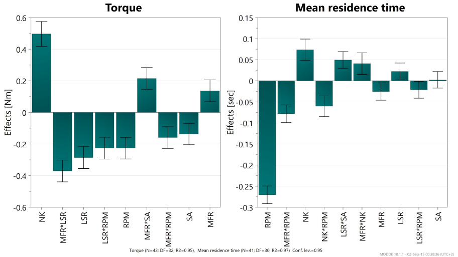
Figure 6.4: Effects plots showing predicted changes in the measured torque and \bar{t} when factors, number of kneading discs (NK) [4, 6, 12], screw speed (RPM) [500-900 rpm], throughput (MFR) [10-25 kg/h], liquid-to-solid ratio (LSR) [6-8%] and stagger angle (SA) [30-60°], vary from low to the high level, while keeping the other factors at their average.
