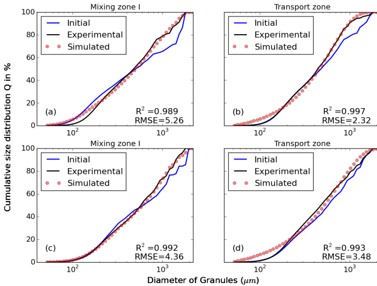
Figure C.1: Fit between the population balance model (PBM) simulated and experimentally measured granule size distribution (GSD) for twin-screw wet granulation with one mixing zone followed by the transport of the granulator at a low (top) and a high (bottom) screw speeds.
