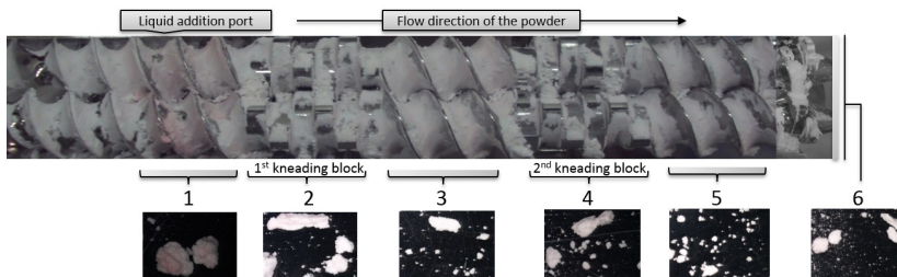
Figure 5.2: Screw configuration with 12 kneading discs (2 blocks) used in the twin screw granulator during the study. Sampling locations along the screw length: [1] before first kneading block, [2] on the first kneading block [3] between first and second kneading block, [4] on the second kneading block [5] after second kneading block, [6] outlet of the granulator.
