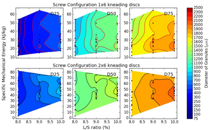
Figure 9.8: Regime map indicating change in percentile values ( D_{25} , D_{50} , D_{75} ) of the granule size distribution with change in L/S ratio and specific mechanical energy input.
