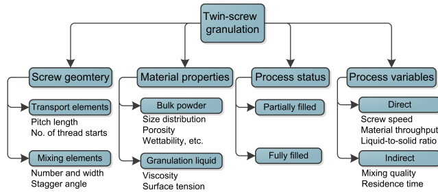
Figure 2.4: Key parameters for measurement and modelling of a twin-screw granulator.
