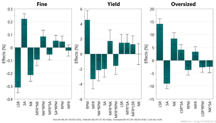
Figure 6.10: Effects plots showing predicted changes in the fines ( >150 \mu\text{m} ), yield [ 150\text{-}1400 \mu\text{m} ] and oversized ( >1400 \mu\text{m} ) fractions of the resulting GSD produced when factors, number of kneading discs (NK) [4, 6, 12], screw speed (RPM) [500-900 rpm], throughput (MFR) [10-25 kg/h], liquid-to-solid ratio (LSR) [6-8%] and stagger angle (SA) [30-60°], vary from a low to a high level, while keeping the other factors at their center point value.
