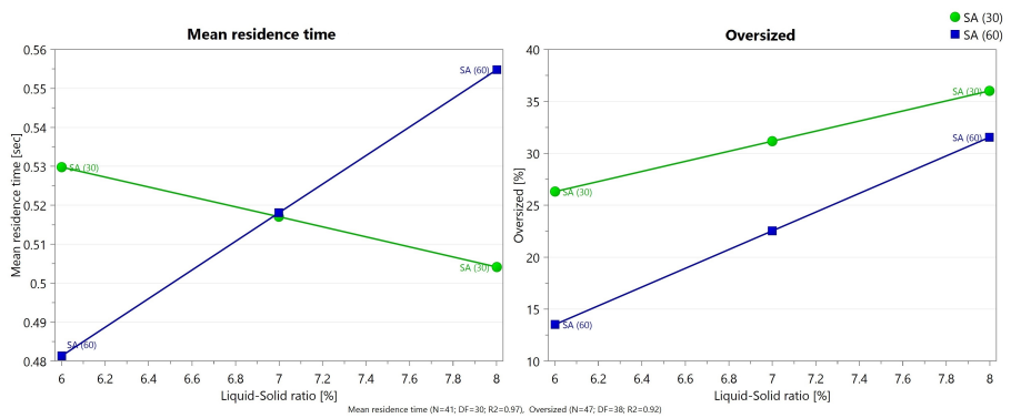
(b) Predicted changes in the mean residence time, and oversized granule fraction (>1400 μm).
