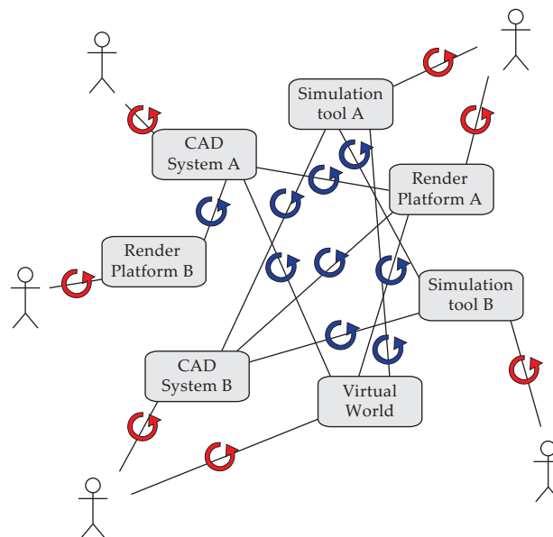
Figure 1. A schema of the typical process of information exchange in an architecture, engineering and construction (AEC) project, with human users in the outer circle, information systems in the inner circle, and connection lines displaying information exchange routes. Interface points (circular arrows) are points where information is interpreted from one information structure into the other, both between human users and information systems (in red) and among information systems (in blue).
