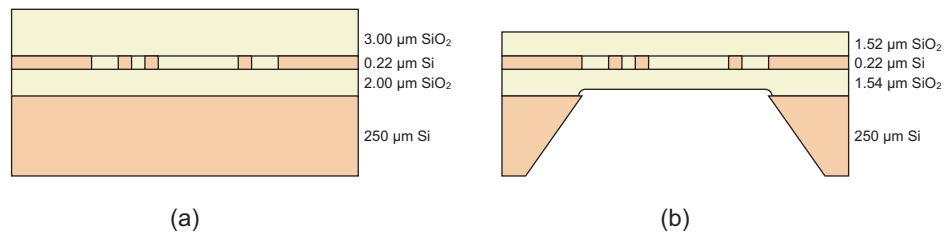
Fig. 2. (a) Initial and (b) final layer stack of the pressure-sensitive membrane.
