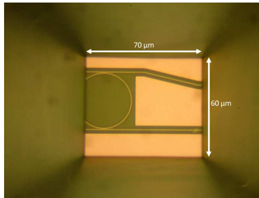
Fig. 4. Microscope image of an underetched ring resonator on a membrane, seen through a hole in the substrate. Dimensions are 60\ \mu\text{m} \times 70\ \mu\text{m} (length \times width).
