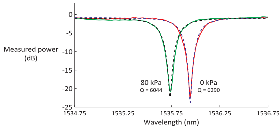
Fig. 5. Measurements of a resonance of a ring resonator are shown here (solid line) along with their fitted Lorentzian shape (dashed line) for a pressure of 0 kPa and 80 kPa. A clear shift is visible with only very slight degradation of the quality factor.
