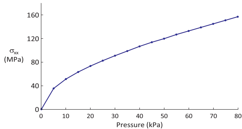
Fig. 1. The non-linear response of the in plane stress \sigma_{xx} in the center of the membrane to the applied pressure.
