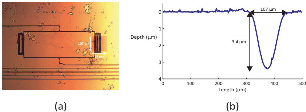
Fig. 7. (a) Microscope image of a Mach-Zehnder interferometer with two waveguide spiral arms as seen from the top side. The right arm is underetched and acts as a pressure-sensitive membrane with dimensions of 107 \mu\text{m} \times 98 \mu\text{m} (length \times width). (b) Measurement of the buckling depth using a Dektak profilometer (buckling depth is 3.4 \mu\text{m} ).
