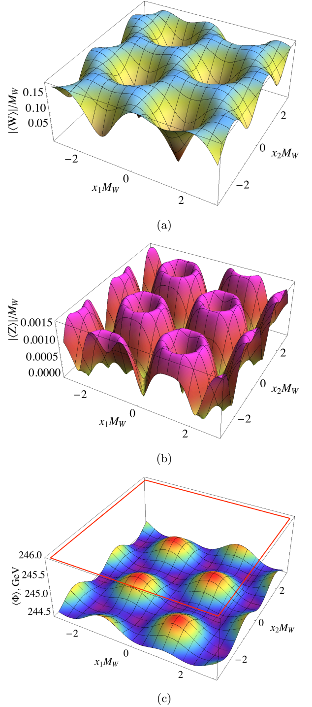
FIG. 2. (a) The superconducting W condensate (16); (b) the superfluid Z condensate (19); (c) the Higgs expectation value (20) as a function of the transverse plane coordinates x_1 and x_2 at the physical Higgs mass M_H = 125 GeV [19] in the background magnetic field B = 1.01B_c^{\text{EW}} directed along the x_3 axis. The red line in figure (c) corresponds to the standard (coordinate-independent) Higgs expectation value, \phi = v/\sqrt{2} , at zero magnetic field B = 0 .
