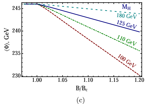
FIG. 1. (a) The cell-averaged W condensate \langle|W|^2\rangle^{1/2} ; (b) the condensation energy density (7), \delta E = \langle E \rangle_W - \langle E \rangle_{W=0} and (c) the cell-averaged Higgs expectation value \langle\Phi^\dagger\Phi\rangle^{1/2} , Eq. (20), vs. the strength of the magnetic field B (in units of the critical magnetic field B \equiv B_c^{\text{EW}} ). The plots are given for various Higgs masses M_H including the physical value of the Higgs mass (the latter are shown by the solid lines).
