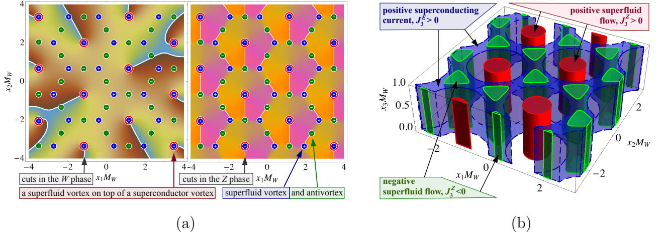
FIG. 3. Kaleidoscopic ground state. Figure (a): The density plots of (the left panel) the phases of the W condensate (16); and (right panel) the Z condensate (19) in the transversal (x_1, x_2) plane at B = 1.01 B_c^{EW} . The end points of the cuts in the phases (shown by the circles) are the superconductor vortices and superfluid (anti)vortices, respectively; (b) the three-dimensional regions of space predominantly occupied by the superconducting electric current J_3^E of the W bosons and the superfluid neutral flows J_3^Z of the Z bosons generated by a weak test electric field E_{\text{ext}} > 0 parallel to the strong magnetic field B = 1.01 B_c^{EW} .
