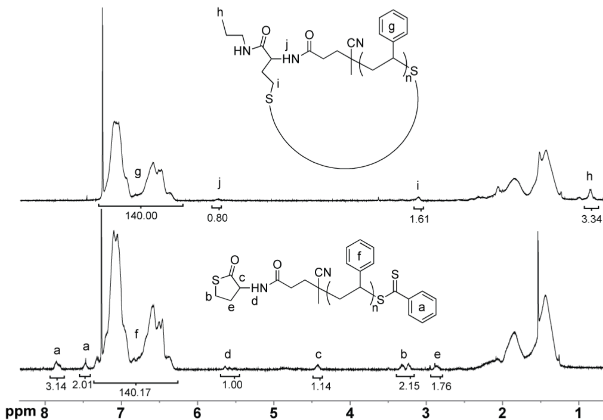
Figure 4. ^1\text{H-NMR} (500 MHz, \text{CDCl}_3 ) spectra of linear PS ( l -PS, 6 , bottom) and cyclic PS ( c -PS, 7a , top) with corresponding signal integration values.
