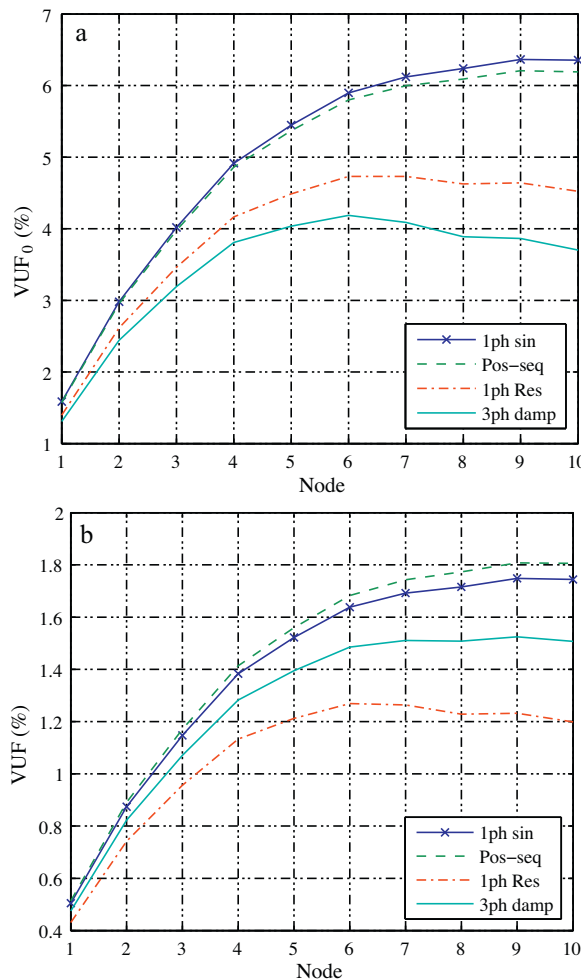
Fig. 8. Simulation A—two three-phase DG-units at node 8 and 10.
