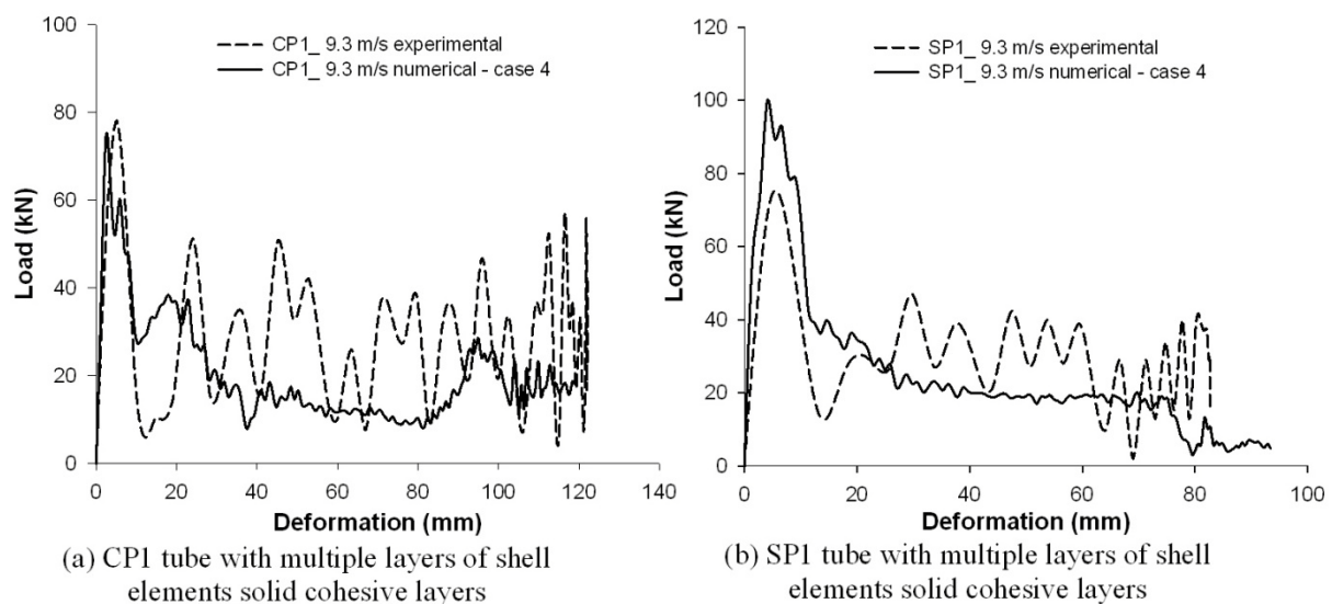
Figure 5: Comparison of load-deformation curve of CP1 and SP1 tubes with multiple layers of shell elements and solid cohesive layers.
