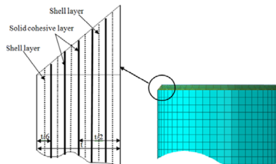
Figure 4: Finite element modelling of CP1 tube series with multiple layers of shell elements and solid cohesive layers.
