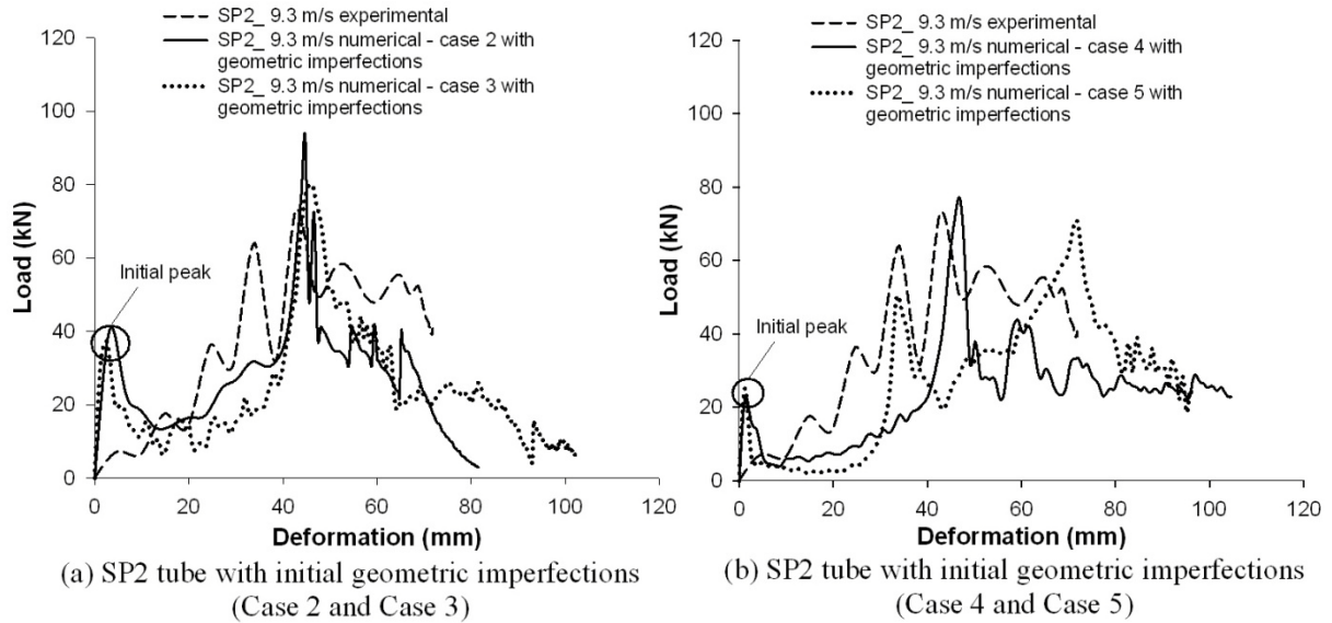
Figure 13: Comparison of load - deformation histories of SP2 tube with initial geometric imperfections.
