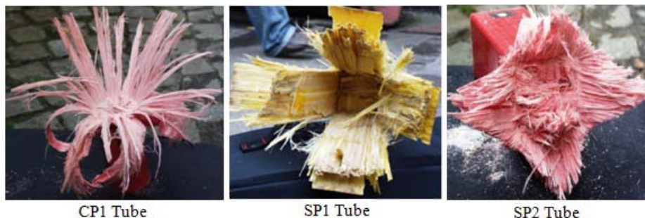
CP1 Tube SP1 Tube SP2 Tube (a) Experimental deformation patterns of different composite tube series.
