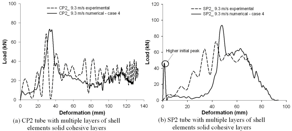
Figure 6: Comparison of force-deformation curve of CP2 and SP2 tubes with multiple layers of shell elements and solid cohesive layers.
