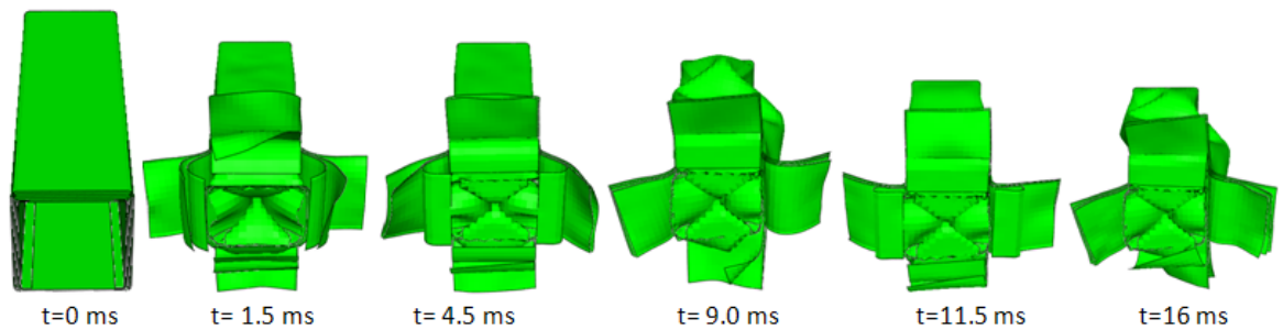
(b) SP1 tube with multiple layers of shell elements, solid cohesive layers and with 4 seams.
