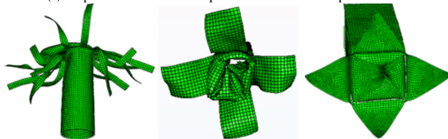
CP1 Tube SP1 Tube SP2 Tube (b) Numerical deformation patterns of composite tubes with two layers of shell elements, cohesive elements and seams (Case 3).
