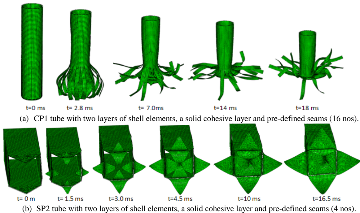
Figure 1: Deformation sequence of CP1 and SP2 tubes with two layers of shell elements, a solid cohesive layer and pre-defined seams.
