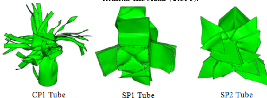
CP1 Tube SP1 Tube SP2 Tube (b) Numerical deformation patterns of composite tubes with two layers of shell elements, cohesive elements and seams (Case 3).
