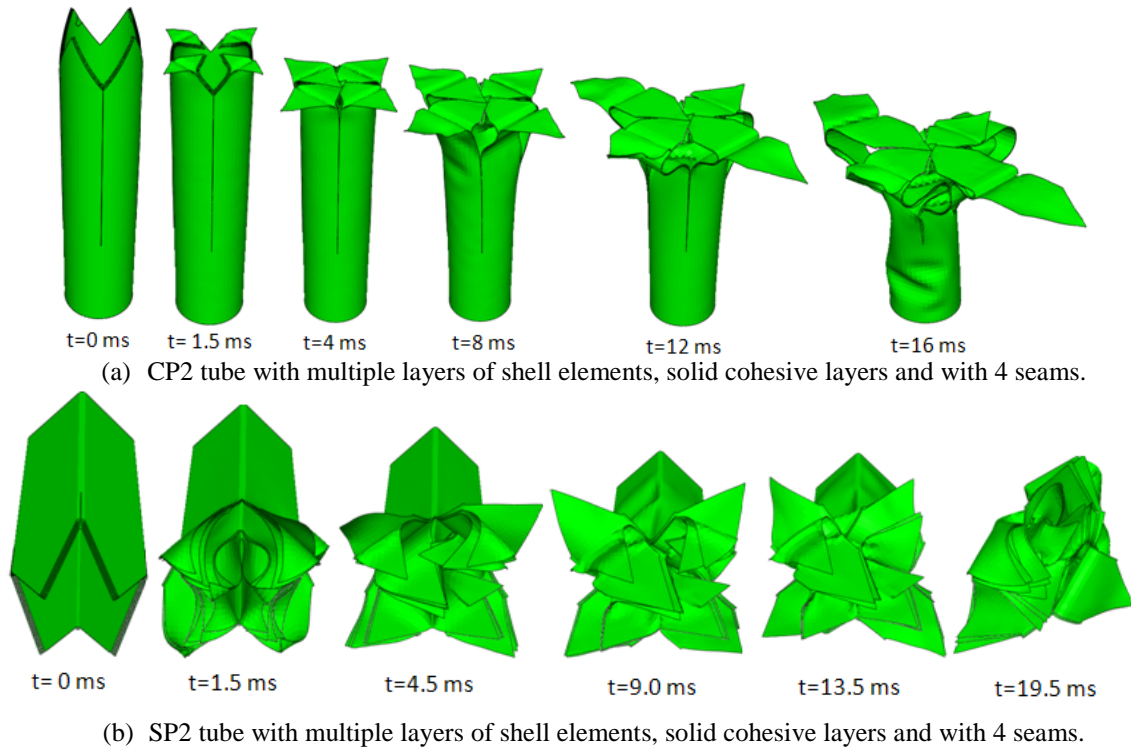
Figure 9: Deformation sequence of CP2 and SP2 tubes with multiple layers of shell elements, solid cohesive layers and with pre-defined seams.
