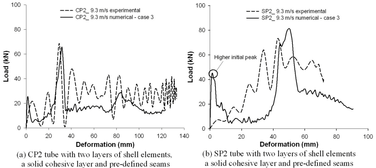
Figure 3: Comparison of load-deformation curve of CP2 and SP2 tubes with two layers of shell elements, a solid cohesive layer and pre-defined seams.
