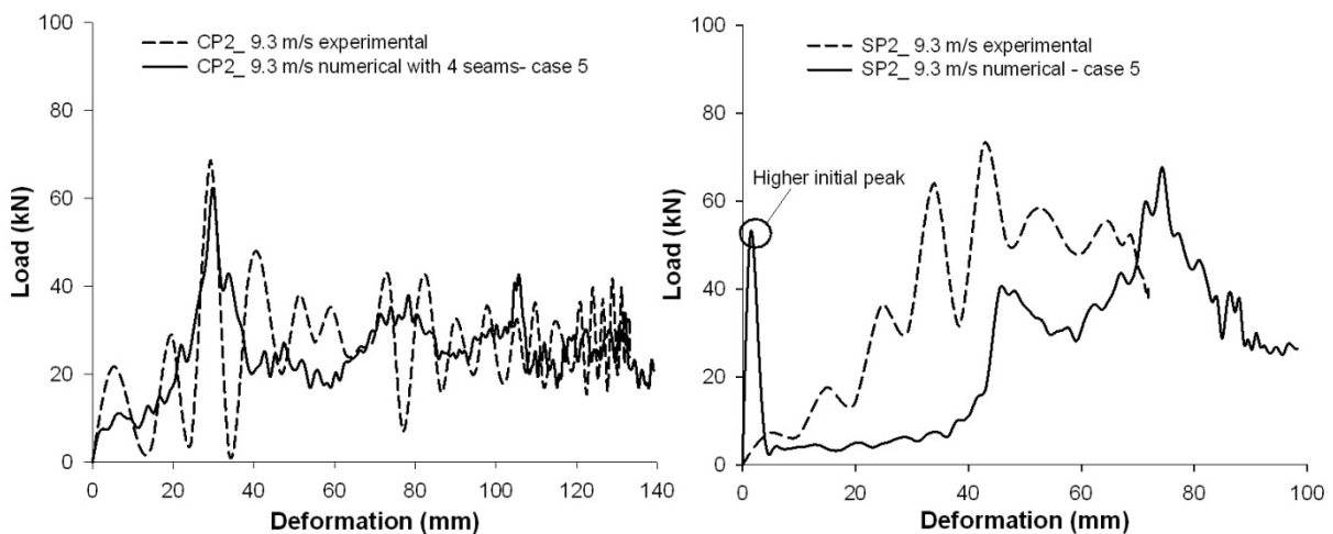
Figure 10: Comparison of load-deformation curve of CP2 and SP2 tubes with multiple layers of shell elements, solid cohesive layers and with pre-defined seams.
