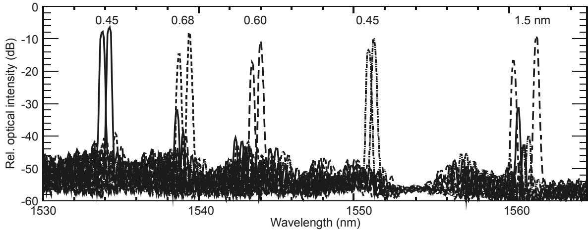
Fig. 8. Spectra showing the upper and lower limits of the five supermodes. The continuous tuning range of each supermode is indicated in the upper part of the image.
