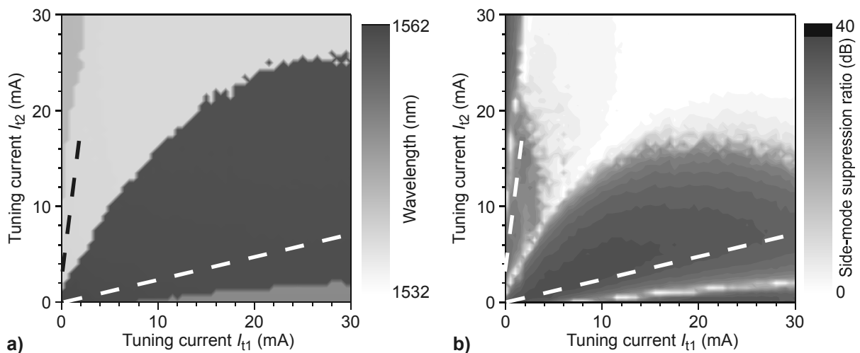
Fig. 7. Tuning behavior of emission wavelength (a) and SMSR (b) of an SG-TTG laser. The dashed lines indicate the tuning curves shown in Fig. 9.
