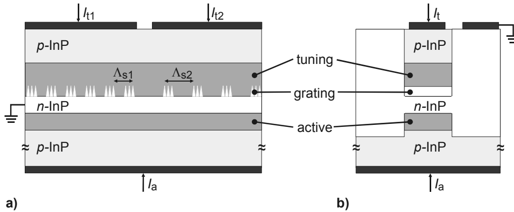
Fig. 1. Schematic drawings of a widely tunable SG-TTG laser diode. a) longitudinal cross-section, b) transverse cross-section.
