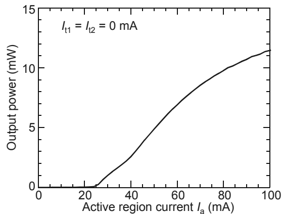
Fig. 6. L-I characteristics of an SG-TTG laser diode.
