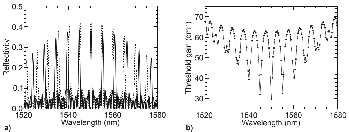
Fig. 2. a) Calculated reflection spectra of SGs with slightly different sampling periods. b) Cavity modes of the corresponding SG-TTG laser diode (dots indicate the position of the cavity modes, lines are only shown as a guide to the eye).
