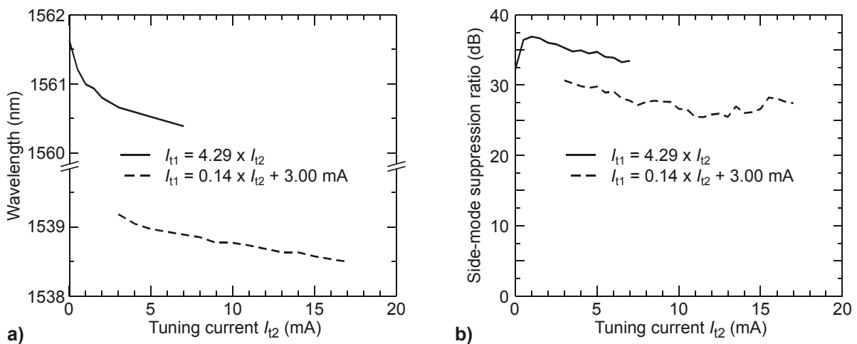
Fig. 9. Variation of emission wavelength (a) and SMSR (b) during continuous tuning (for two selected supermodes, shown as dashed lines in Fig. 7).
