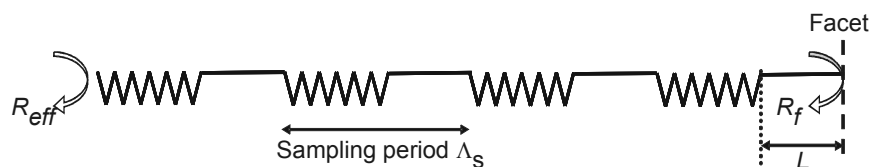
Fig. 3. The effective reflectivity R_{eff} of one grating section is determined by the interference of reflections from the sampled gratings and from the facet, which is situated a distance L away from the grating.
