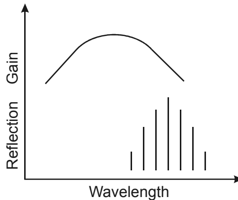
Fig. 10. Detuning of gain peak and SG reflection spectrum.
