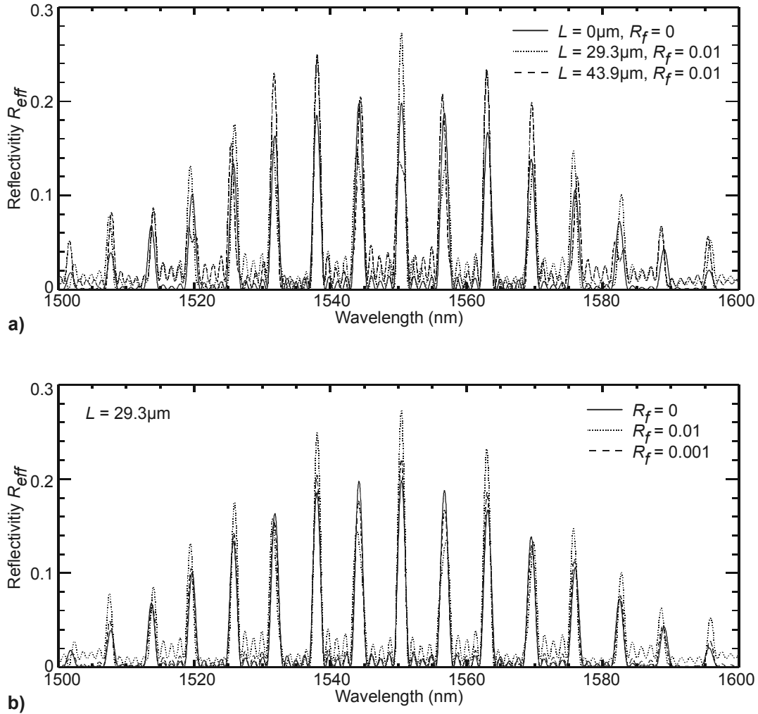
Fig. 4. Reflection spectra of a sampled grating section that interferes with a facet of reflectivity R_f , which is separated from the sampled grating by a distance L .
