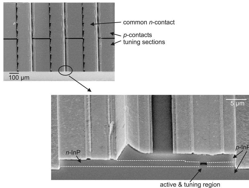
Fig. 5. SEM images showing an SG-TTG laser chip. The dashed white lines in the lower image indicate the location of the InP p - n -homojunctions. The common n -contact is situated on the left hand side of the ridge and the electron current is injected into the active and tuning regions via the n -InP channel.
