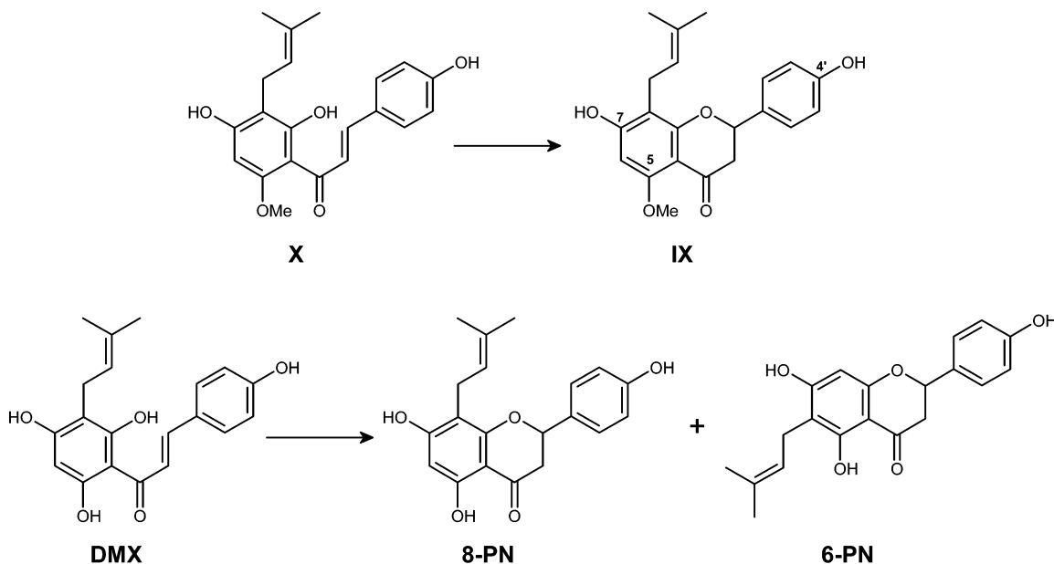
Figure 1. Structures of hop prenylflavonoids. By thermal isomerization, the chalcones X and DMX are converted into the respective flavanones IX (from X) and 8-PN and 6-PN (from DMX).
