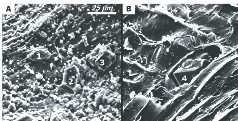
Figure 5. Scanning electron microscopical observations made on small samples at 654× magnification: (A) three fragmented crystalloid particles (labels 1 to 3) and amorphous granules (e.g. white arrow) surrounded by debris, on the sample surface; (B) free, fairly intact, large crystal found lodged inside a parenchyma ray cell that had been cut open during sample preparation (label 4). The 25 µm scale bar is valid for both SEM photographs.
