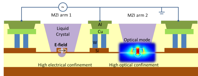
Fig. 1. Conceptual drawing the device under test.
