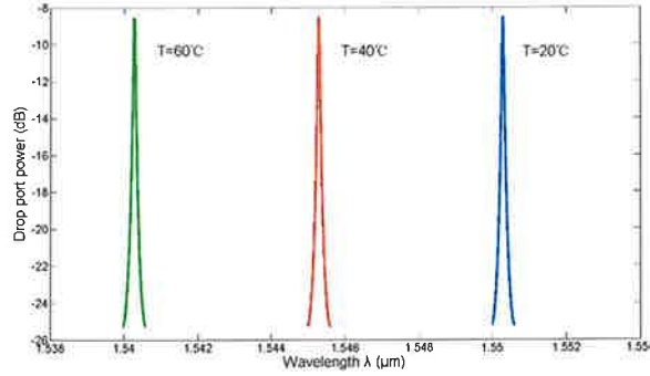
Fig.2 Transmission spectra from drop port of microring resonator with silicon substrate and water up-cladding at different temperatures
