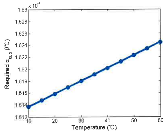
Fig.3 Required TEC of substrate for athermalization at different temperatures
