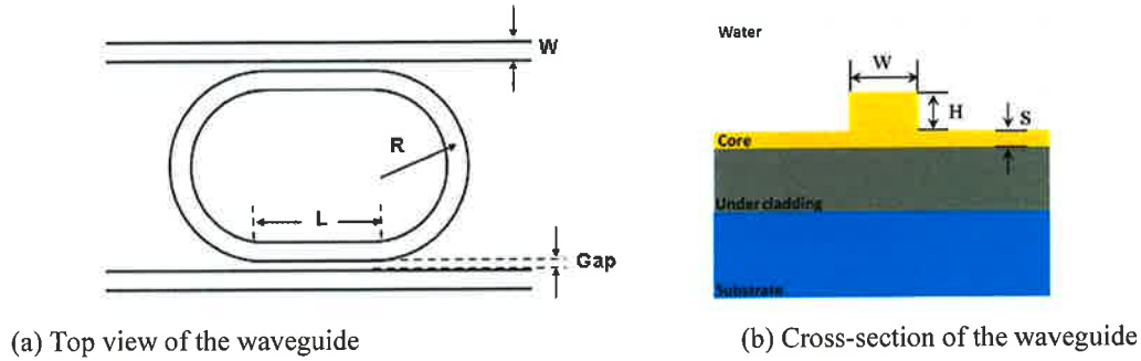
Fig.1 Schematic structure of racetrack waveguide microring resonator
