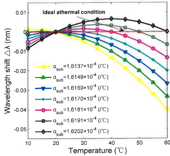
Fig. 4 Resonant wavelength shift versus temperature with different substrate TECs
