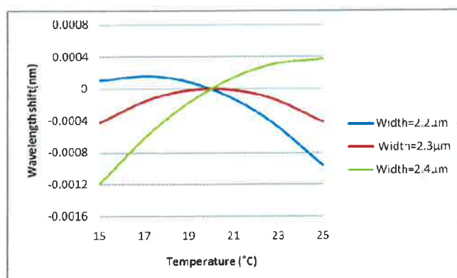
Fig. 5 Resonant wavelength shift versus temperature for different waveguide widths
