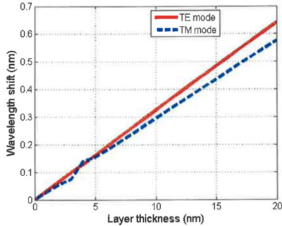
Fig. 7 The resonant wavelength shift of the MRR with the thickness of biomolecular layer.
