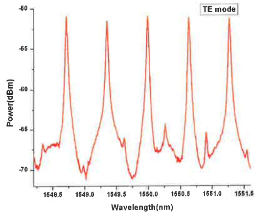
Fig. 9 The transmission of the microring resonator at the drop port for TE mode.
