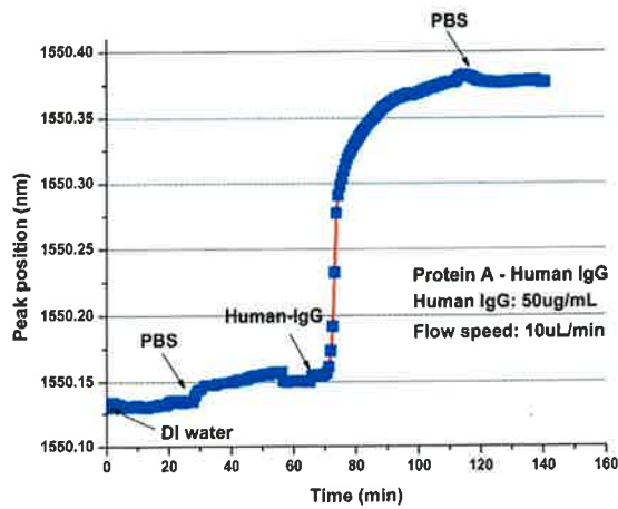
Fig. 10 Real-time monitoring of the resonance peak of the microring resonator-based sensor with the flowing human-IgG solution.
