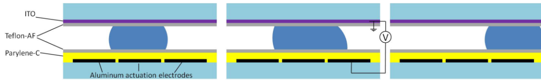
Figure 1. A diagram of the cross-section of an EWOD lab-on-a-chip and the electrowetting principle. When a voltage is applied to an actuation electrode, the droplet is attracted toward this activated region due to the generated imbalance in interfacial tension near the surface above the actuated electrode [2].
