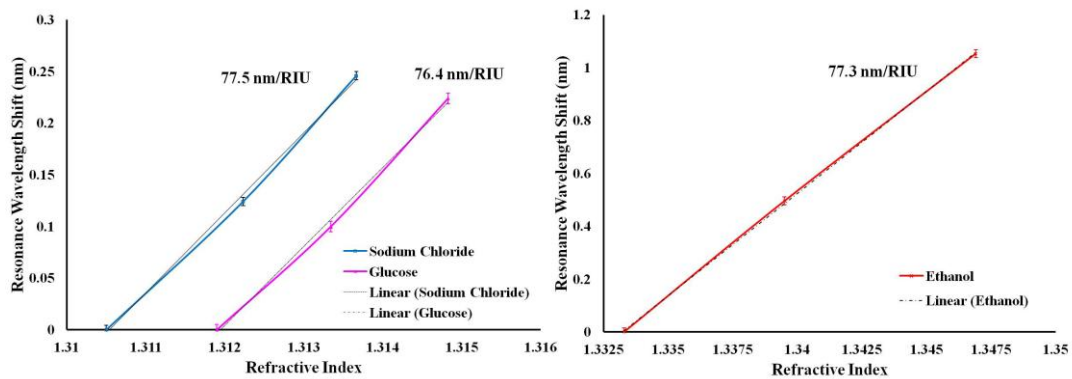
Figure 4. Three experiments with different sodium chloride, glucose and ethanol concentrations were performed. Each line corresponds to one of these experiments. Error bars indicate the standard deviations based on 3 repetitions. The sensitivity is determined to be 77 \pm 0.6 nm/RIU [4].
