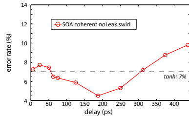
Figure 1. Result of a network of SOAs with a different delay in between them on a isolated digit recognition task
