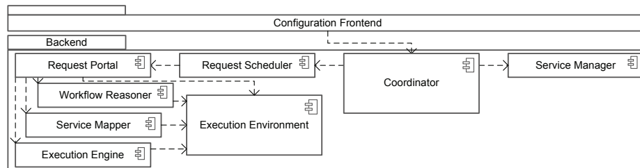
Fig. 1. Main building blocks of the mashup creation and execution framework.
