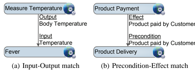
Fig. 4. Semantic match between two service interfaces.
