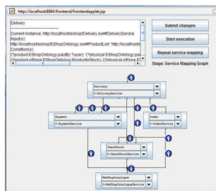
Fig. 3. Configuration Frontend, showing a composite mashup graph.
