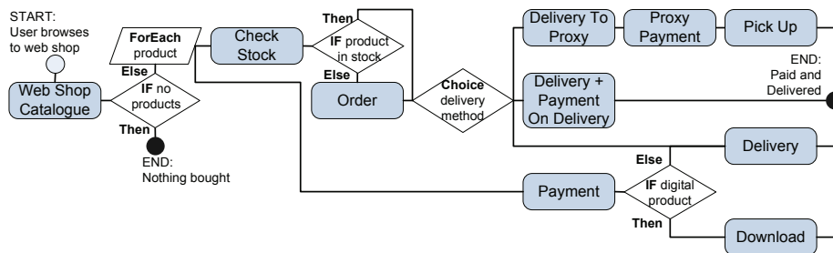
Fig. 6. Constructed e-shop workflow with the use of control constructs.
