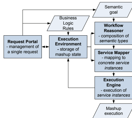
Fig. 2. Mashup creation, execution and runtime adaptation process for a user's request.
