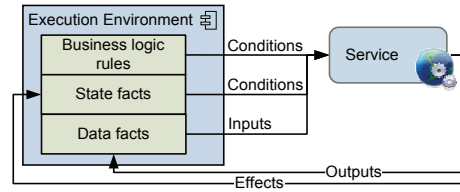
Fig. 5. Inference through matching of service preconditions and inputs and returning service effects and outputs.
