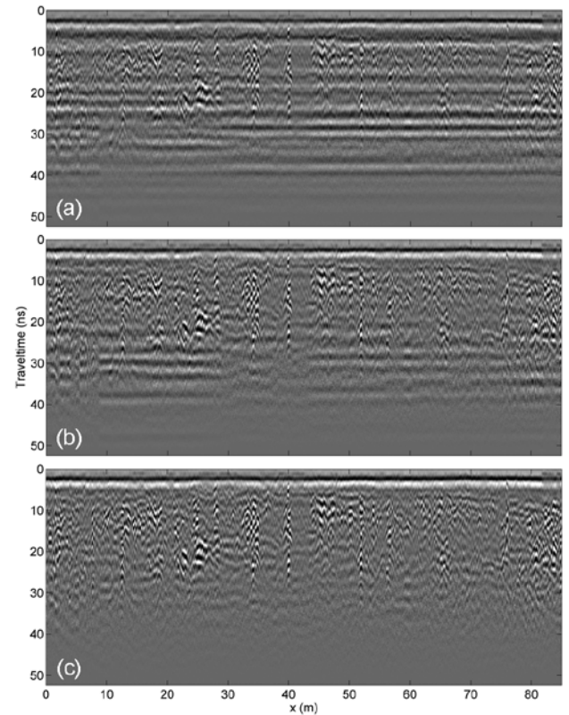
Figure 6. GPR profile showing ringing noise. (a) Raw data. (b) The same profile after background removal. (c) The same profile after application of a combined fan filter and circular filter in the three-dimensional f - k domain.
