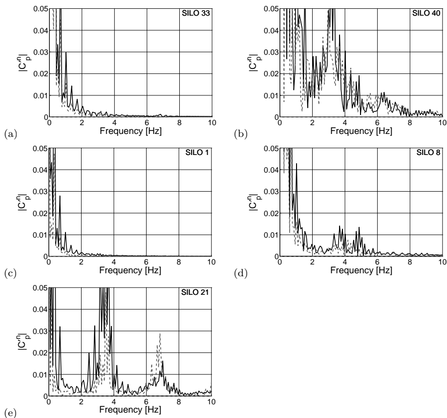
Figure 7: Frequency spectra for the amplitude of C_p'^3 (solid line) and C_p'^4 (dashed line) for angle of incidence \alpha = 30^\circ for (a) cylinder 33, (b) cylinder 40, (c) cylinder 1, (d) cylinder 8 and (e) cylinder 21.
