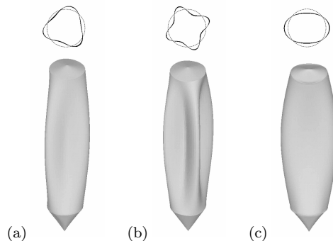
Figure 2: Selected ovalling eigenmodes of a single silo, (a) mode (1,3) at 3.93 Hz, (b) mode (1,4) also at 3.93 Hz and (c) mode (1,2) at 7.75 Hz [3].
