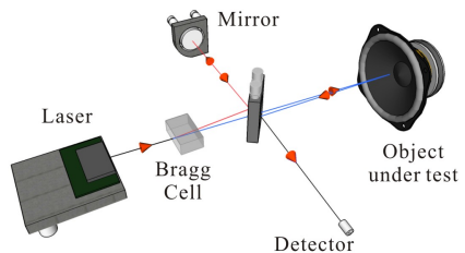
Figure 1. Illustration of a commercialized bulk LDV system with a heterodyne interferometer. The laser is split into two beams: the reference beam (frequency shifted) and the measurement beam (no previous frequency shift). The reflected measurement beam is mixed with the reference beam at the photo-detector, where the detected signal is sent to the decoder for demodulation.
