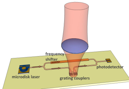
Figure 2. The miniaturized laser Doppler velocimetry on SOI. The laser is generated by a bonded micro-disk laser, and split into a measurement and a reference signal. The measurement signal is sent out and captured through grating couplers and reflected back by the moving target. The reference signal is mixed with the captured measurement signal after being frequency shifted by an optical frequency shifter. The photo-detector, which is also integrated on SOI substrate by BCB bonding, detects the combined signal and sends it to the decoder.
