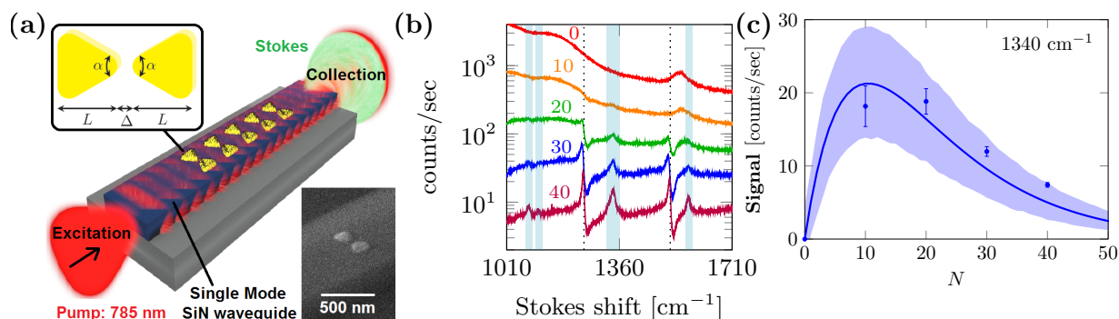
Fig. 1: (a) Silicon nitride (SiN) waveguide functionalized with an array of N bowtie antennas. The bottom inset shows a SEM image of an integrated bowtie antenna. (b) SERS spectra of waveguides functionalized with a varying number of N ( N = 0, 10, 20, 30, 40 ) bowtie antennas with \alpha \approx 60^\circ , L \approx 106 \pm 8 nm and \Delta \approx 48 \pm 13 nm. (c) Signal strength of the 1340 \text{ cm}^{-1} peak as a function of N (points). The solid curve represents a fit of the experimental data to a theoretical model, developed in [3], which describes the on-chip SERS effects. The shaded area incorporates the theoretical impact of disorder in the system [3].
