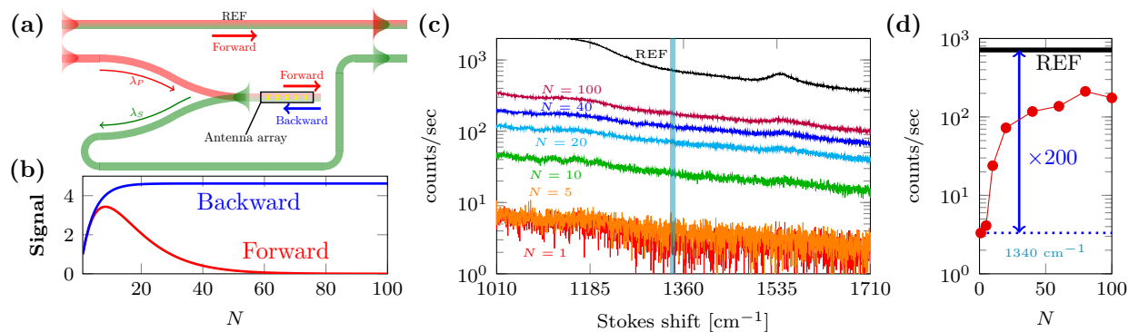
Fig. 2: (a) (top) Straight reference waveguide REF with copropagating pump and Stokes; (bottom) Y-splitter design separating pump and Stokes beam. (b) Theoretical comparison between forward and backward on-chip SERS scattering. (c) Backward scattered Raman spectra of a Y-splitter functionalized with varying N . For comparison, the forward scattered Raman spectrum of a straight reference waveguide (REF) is also added. The cyan shaded area marks the 1340\text{ cm}^{-1} region. (d) Zoom on the background of the 1340\text{ cm}^{-1} region.
