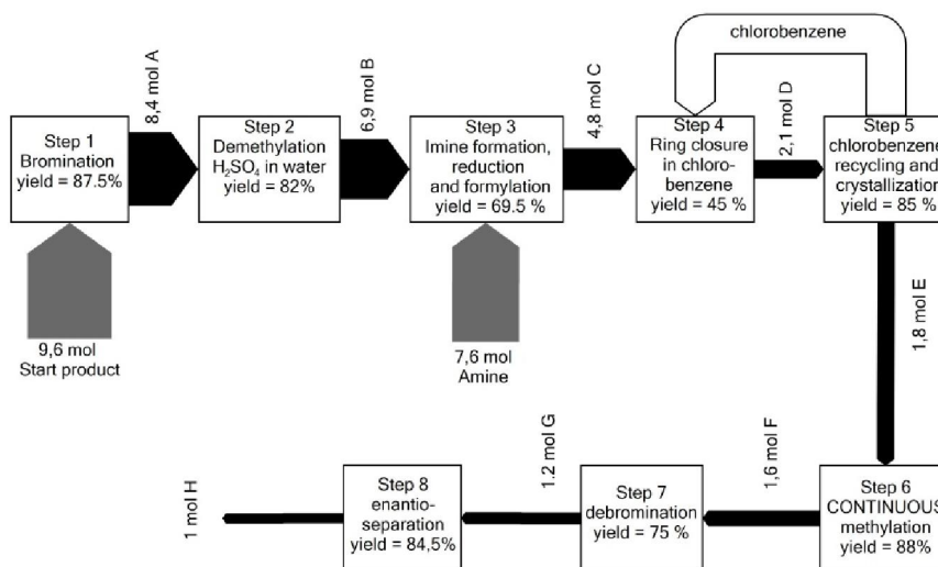
Fig. 2: Synthesis route for the production of 1 mol intermediate H using the continuous process (micro reactor technology) in step 6
