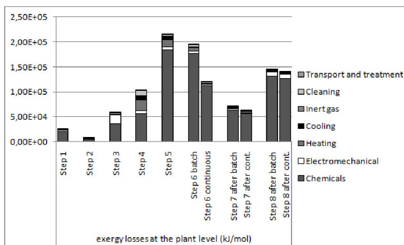
Fig. 6. Non cumulative exergy losses at the plant level for eight consecutive production steps and divided over seven impact categories
