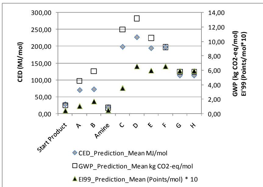
Fig. 5: ETH prediction of ten intermediate molecules in the synthesis route of galantamine
