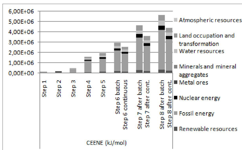
Fig. 8: CEENE of the eight production steps (cumulative results)
