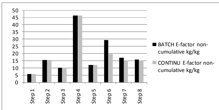
Fig. 3: Non-cumulative E-factor of eight consecutive production steps
