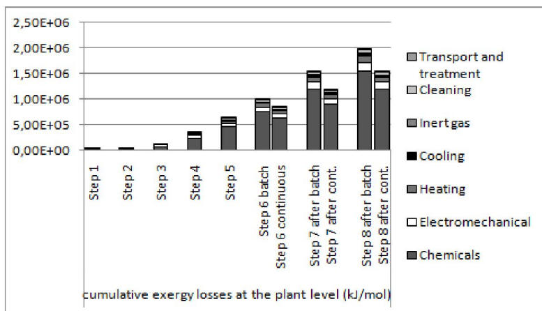
Fig. 7. Cumulative exergy losses at the plant level for eight consecutive production steps and divided over seven impact categories
