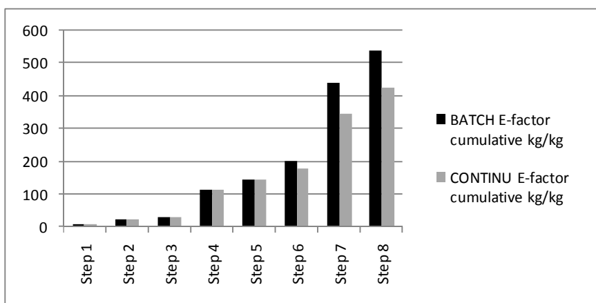
Fig. 4: Cumulative E-factor of eight consecutive production steps
