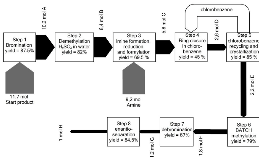
Fig. 1: Synthesis route for the production of 1 mol intermediate H using the batch process in step 6
