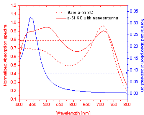
Fig. 2. Normalized absorption spectra of the investigated SC (red lines) and absorption cross-section of the proposed single core-shell antenna (blue line).
