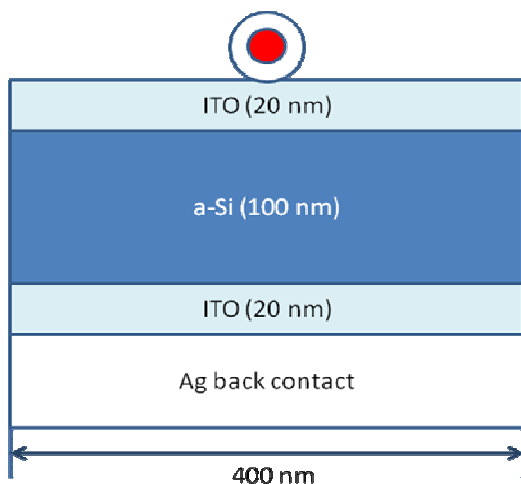
Fig. 1. A cross-section of the investigated SC. (ITO stands for indium tin oxide).
