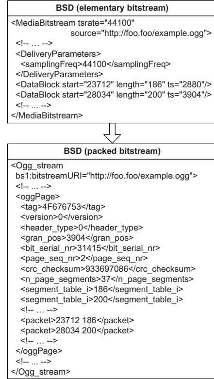
Fig. 8. XML-driven Ogg packaging.
