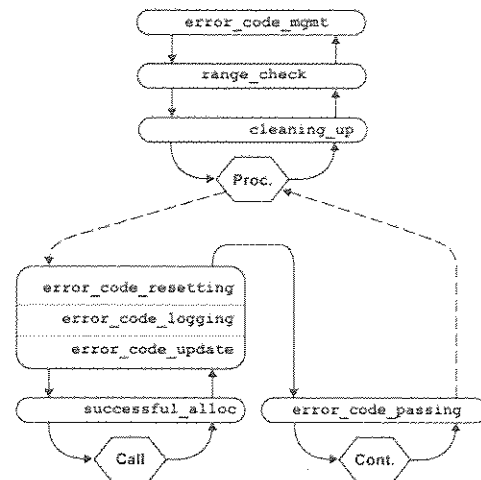
Figure 7. Schematic order of execution of a woven idiomatic procedure. Full arrows denote execution flow, while dashed ones indicate that the sequence in between them can show up zero or more times. Rounded rectangles represent advice, while hexagons indicate execution, call and local continuation join points. The advice name is centered for around-advice, while it is right-aligned for after-advice.
