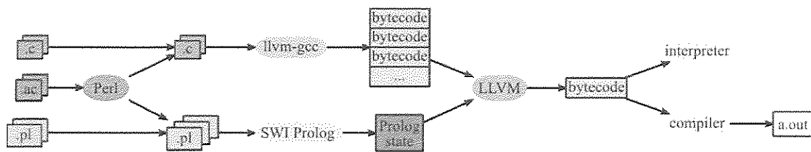
Figure 14. Aspicere2's weaver architecture.
