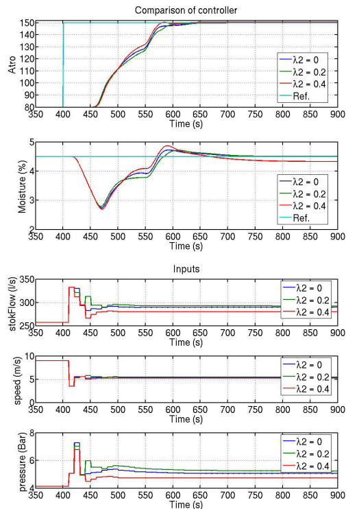
Fig. 2. Behavior of the controller for three different values of \lambda_2 tuning parameter.
