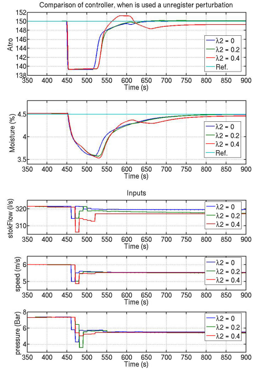
Fig. 3. Behavior of the controller when an unmeasured perturbation was applied in the consistency of the pulp from 1.4 % to 1.3% for three different values of \lambda_2 tuning parameter.
